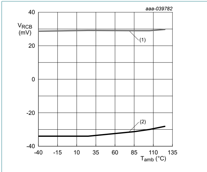
V_{IN} = V_{EN} = 1.2 \text{ to } 5 \text{ V}; V_{OUT} - V_{IN} V_{RCB\_R} (enable) V_{RCB\_F} (disable) (1) (2)
