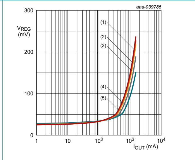
V_{IN} = 3.3 \text{ V}; V_{EN} = 0 \text{ V}; C_L = 100 \text{ nF} -40 °C 25 °C 85 °C 105 °C 125 °C (1) (2) (3) (4) (5)
