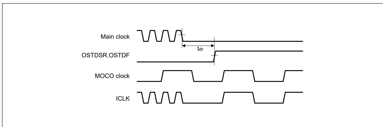
Figure 2.55 Oscillation stop detection timing
