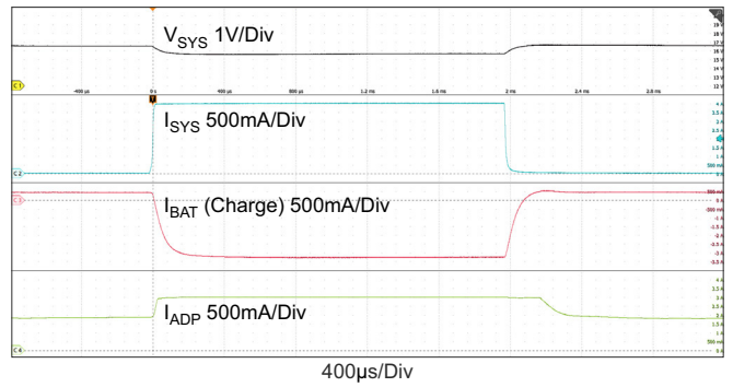
Figure 24. Boost Mode: Charge Current Loop ↔ Adapter Current Loop, V_{ADP} = 5V , MaxSystemVoltage = 21V, V_{BAT} = 16V , AdapterCurrentLimit = 3A, ChargeCurrent = 0.5A, SystemLoad: 0A ↔ 4A
