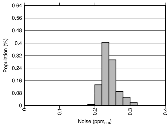
0.1-Hz to 10-Hz Voltage Noise Distribution
