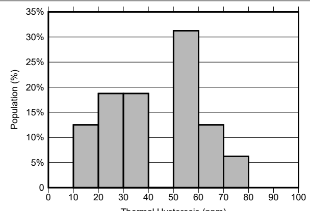
Figure 7-22. REF7025QFKHR Thermal Hysteresis Distribution (0°C to 70°C)
