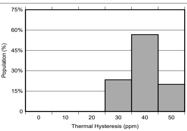
Figure 7-24. REF7012QDGKR Thermal Hysteresis Distribution (0°C to 70°C)
