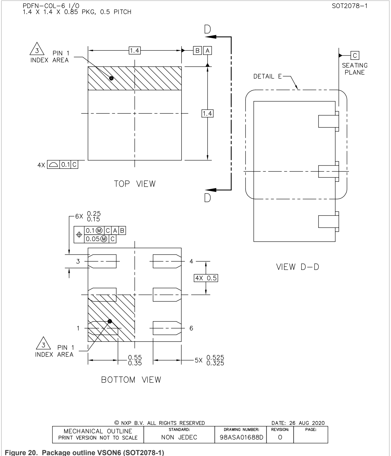
Figure 20. Package outline VSON6 (SOT2078-1)
