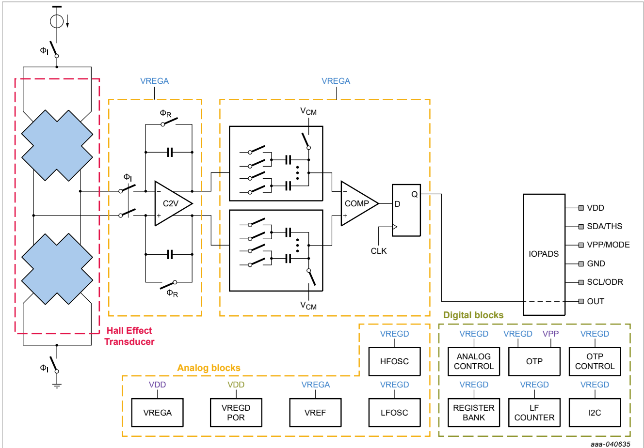
Figure 1. Block diagram
