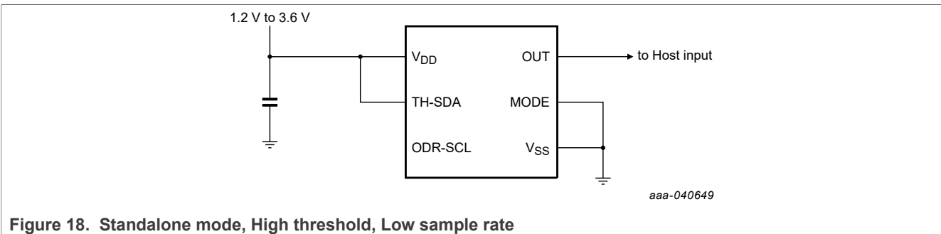
Figure 18. Standalone mode, High threshold, Low sample rate
