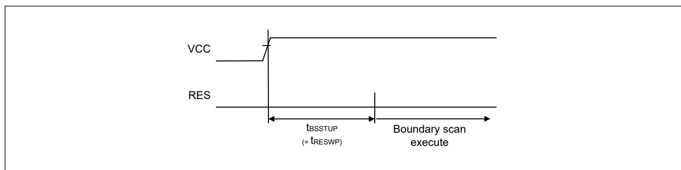
Figure 2.98 Boundary scan circuit startup timing
