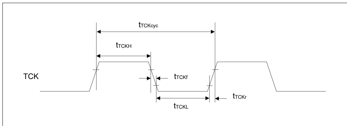
Figure 2.99 JTAG TCK timing
