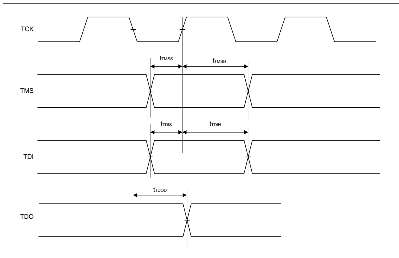
Figure 2.100 JTAG input/output timing
