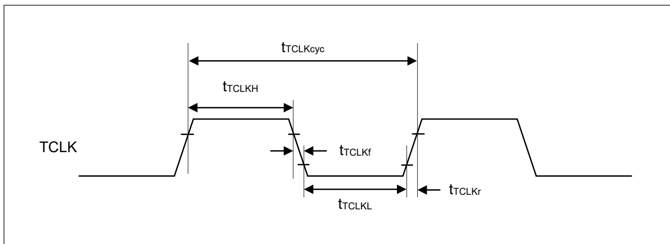
Figure 2.103 ETM TCLK timing
