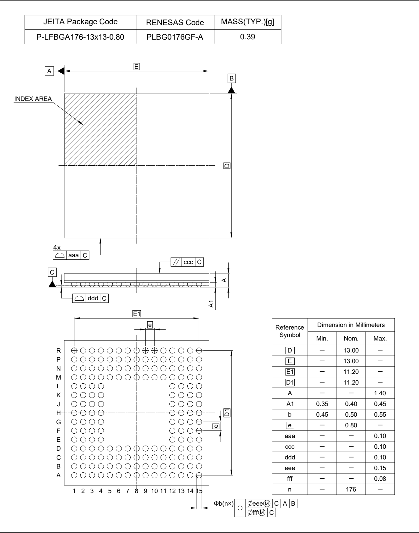
Figure A2.2 BGA 176-pin
