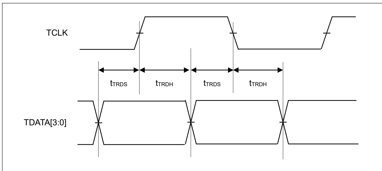
Figure 2.104 ETM output timing
