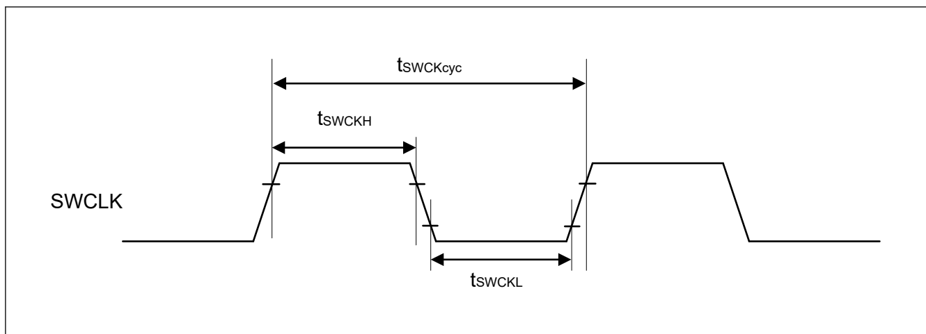
Figure 2.101 SWD SWCLK timing
