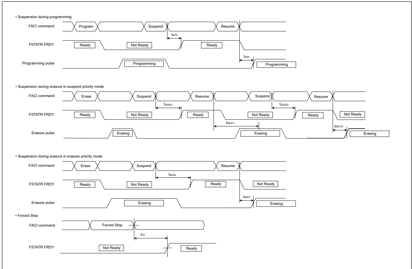
Figure 2.95 Suspension and forced stop timing for flash memory programming and erasure
