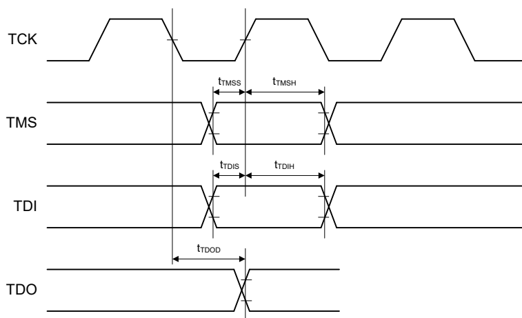
Figure 2.97 Boundary scan input/output timing
