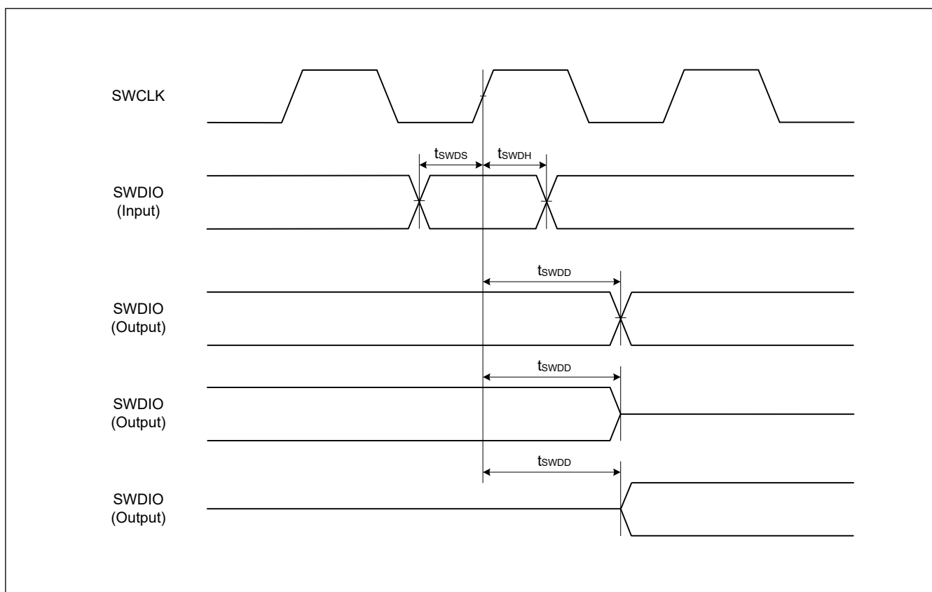
Figure 2.102 SWD input/output timing
