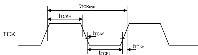
Figure 2.96 Boundary scan TCK timing
