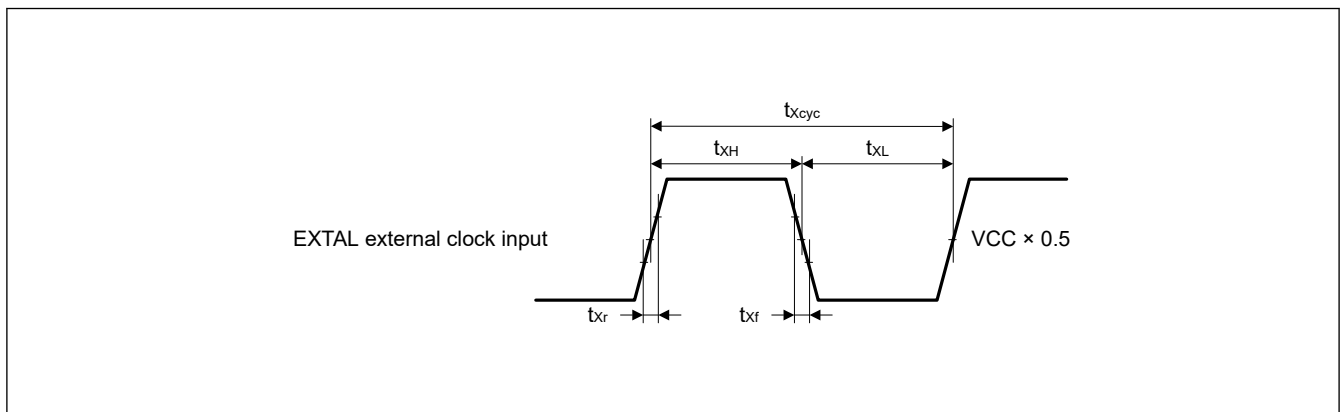
Figure 2.8 EXTERNAL external clock input timing
