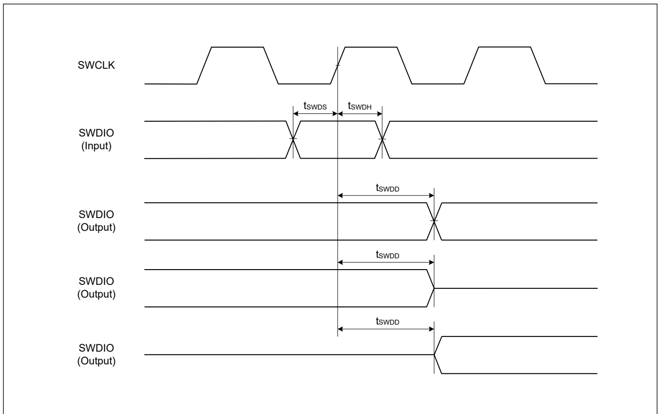
Figure 2.102 SWD input/output timing
