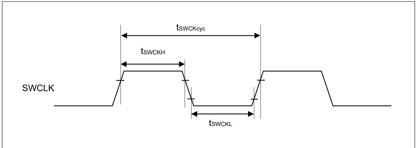
Figure 2.101 SWD SWCLK timing
