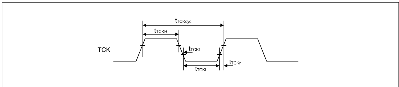
Figure 2.96 Boundary scan TCK timing
