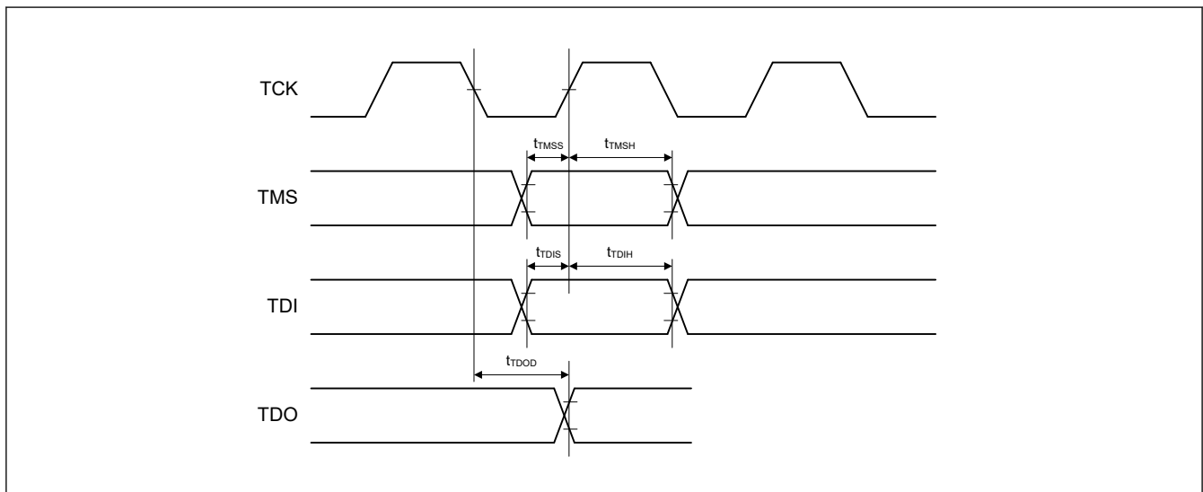
Figure 2.97 Boundary scan input/output timing
