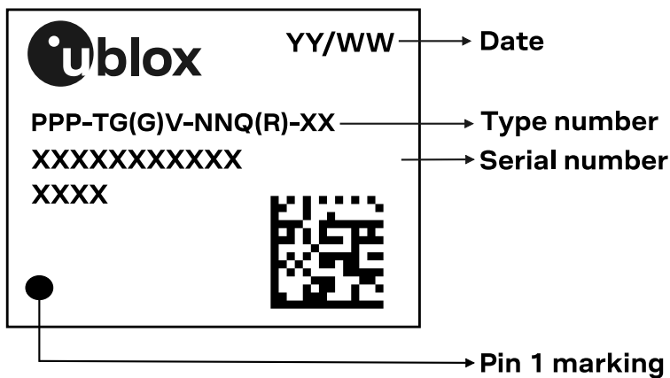
Figure 5: Example of NEO-F10N product marking
