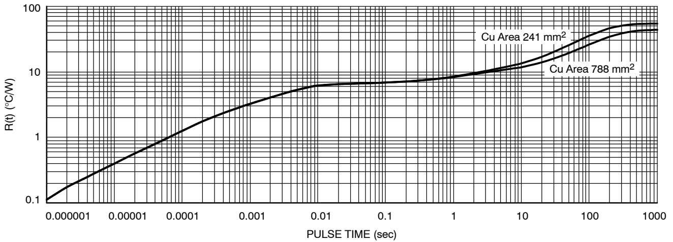
Figure 33. Single-Pulse Heating Curves, D 2 PAK 5-Lead
