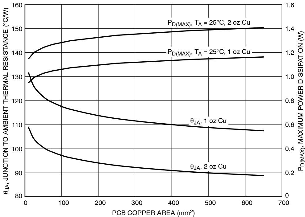
Figure 50. θ JA and P D (MAX) vs. Copper Area (CSP4)
