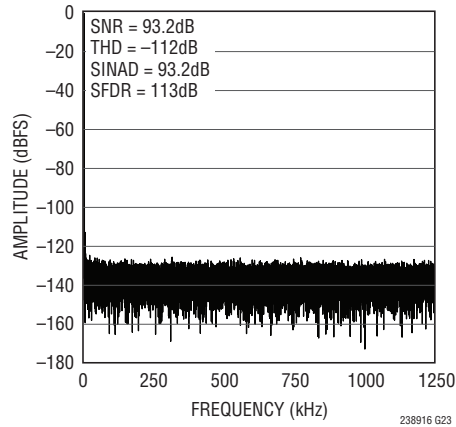
32k Point FFT f_{SAMPL} = 2.5\text{Mpsps} , f_{IN} = 2\text{kHz}
