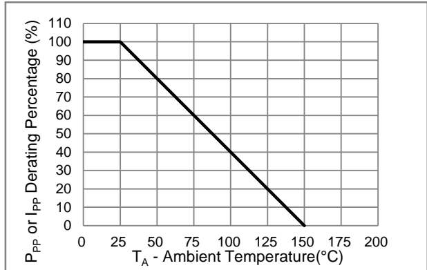
Fig.2 Derating Curve
