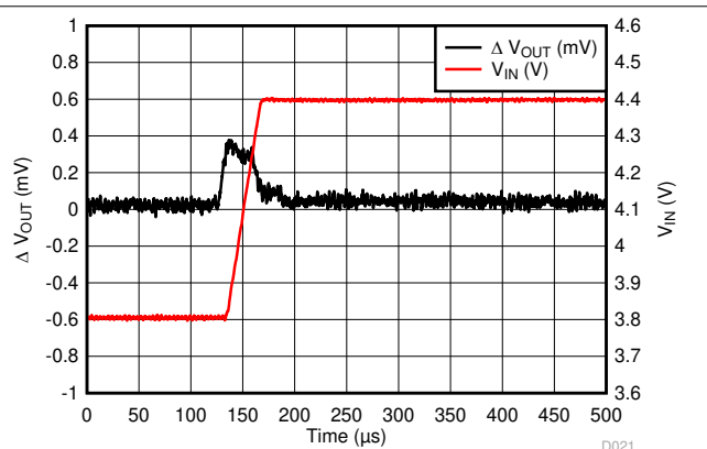
Figure 6-28. LP5912-1.8 Line Transient
