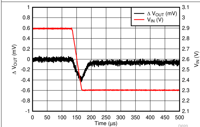
Figure 6-27. LP5912-0.9 Line Transient
