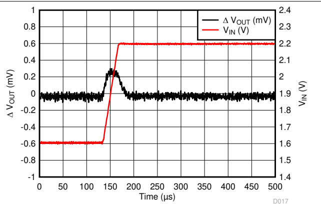
Figure 6-26. LP5912-0.9 Line Transient
