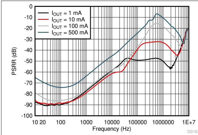
Figure 6-25. LP5912-3.3 PSRR vs Frequency
