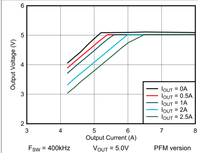
Figure 6-3. 5V Dropout
