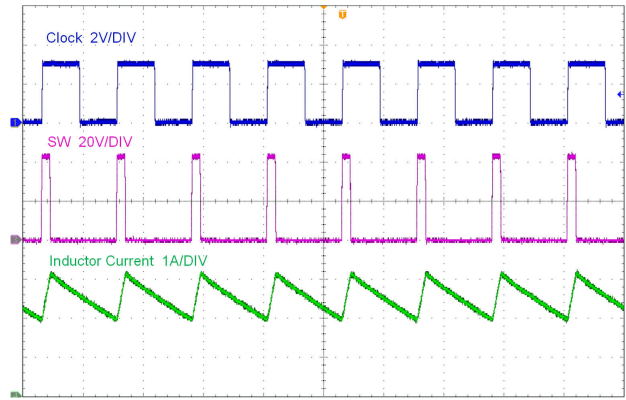
LMR38025 V_{OUT} = 5V 400kHz 2µs/DIV
