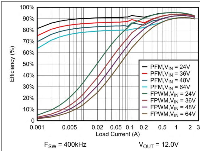
Figure 6-1. Efficiency vs Load Current
