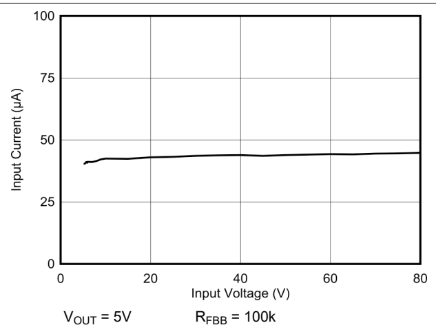
Figure 6-2. No Load Input Current vs Input Voltage
