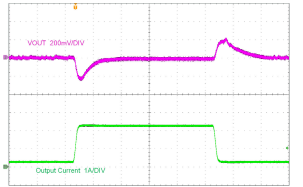
LMR38025(PFM) V_{OUT} = 5V 400kHz, 100µs/DIV (AC Coupled) 250mA to 2.25A at 200mA/µs
