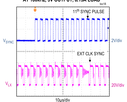
APPLICATION OF EXTERNAL CLOCK AT 180kHz, 5V OUTPUT, 0.15A LOAD
