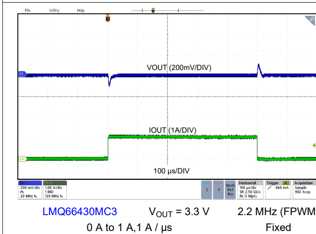
Figure 8-12. Load Transient
