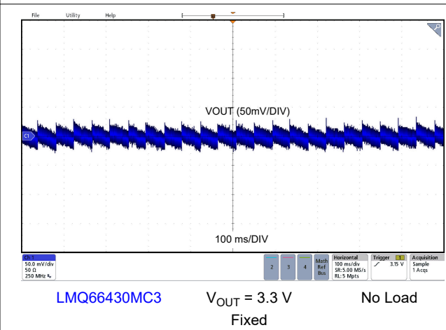
Figure 8-15. Output Voltage Ripple
