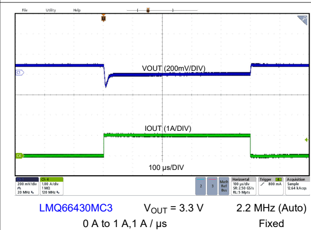
Figure 8-13. Load Transient
