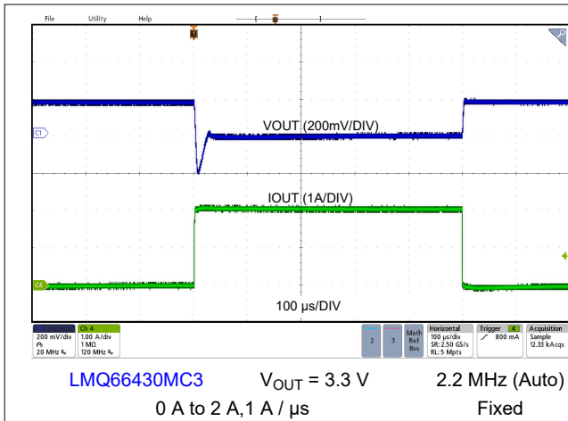
Figure 8-10. Load Transient
