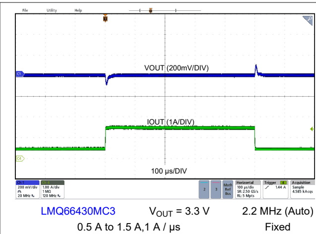
Figure 8-11. Load Transient
