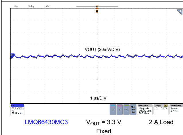
Figure 8-14. Output Voltage Ripple
