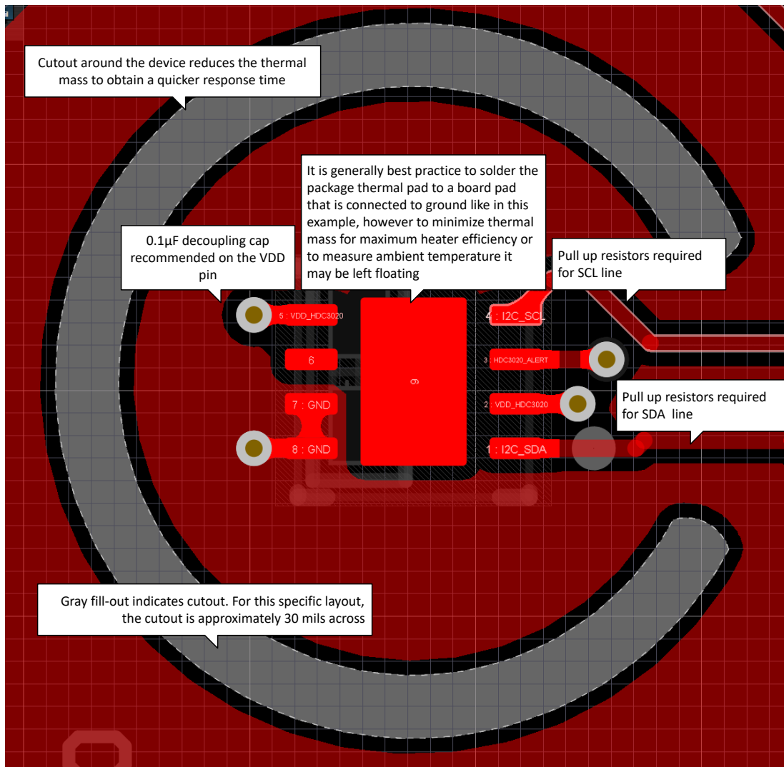
Figure 8-3. HDC302x PCB Layout Example
