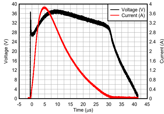
Figure 5-14. 8/20µs Surge Response at 5.7A
