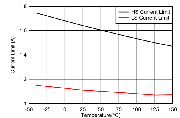
Figure 6-18. HS and LS Current Limit Versus Temperature
