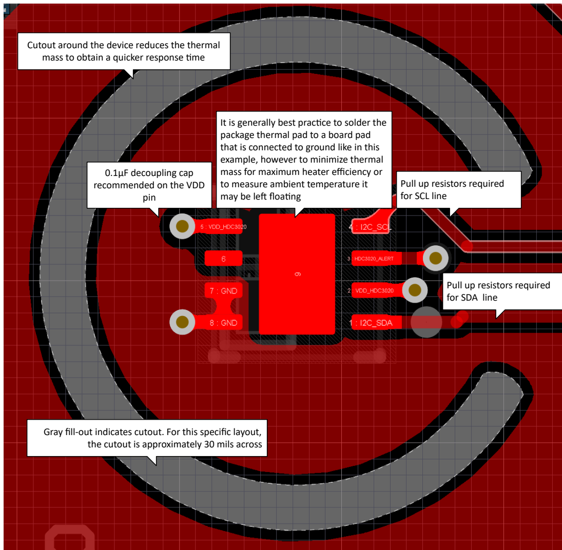
Figure 8-3. HDC302x-Q1 PCB Layout Example
