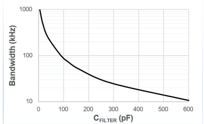
Figure 13: Experimental Bandwidth vs. C_{FILTER}
