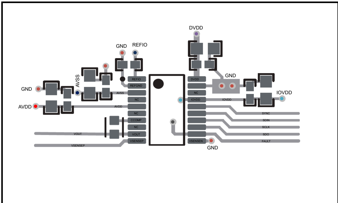
Figure 8-8. Layout Example
