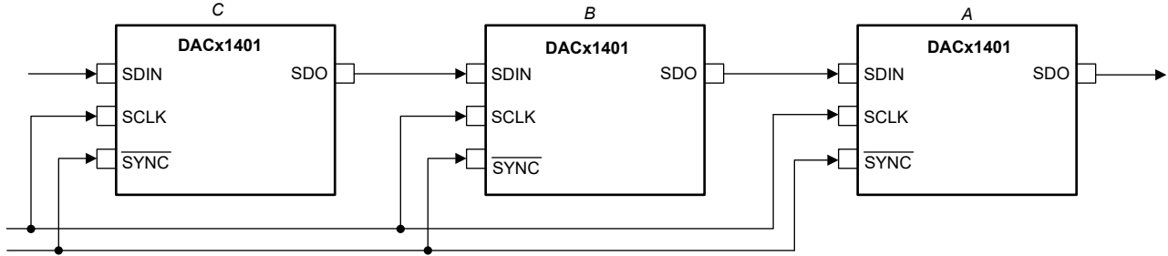
Figure 6-3. Daisy-Chain Setup
