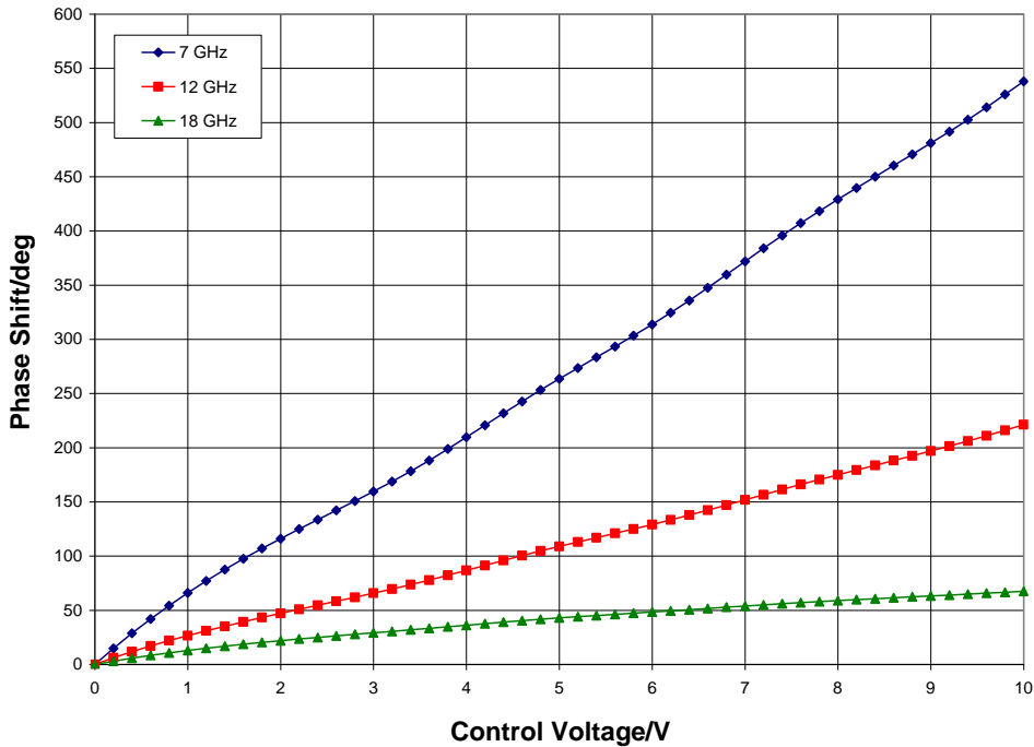
Phase Shift vs. Control Voltage, T A = 25 °C
