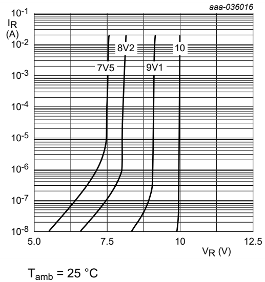
Fig. 6. Reverse current as a function of reverse voltage; typical values (BZX38450-B/C7V5 to BZX38450-B/C10)
