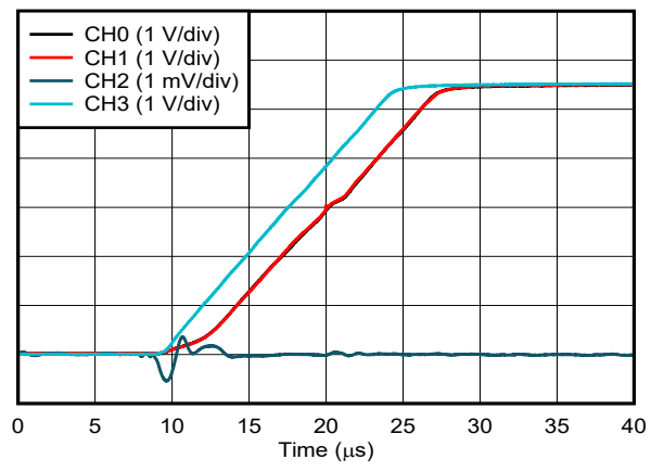
Channel 2 is victim, all other channels are aggressors Figure 6-25. Voltage Output Channel-to-Channel Crosstalk
