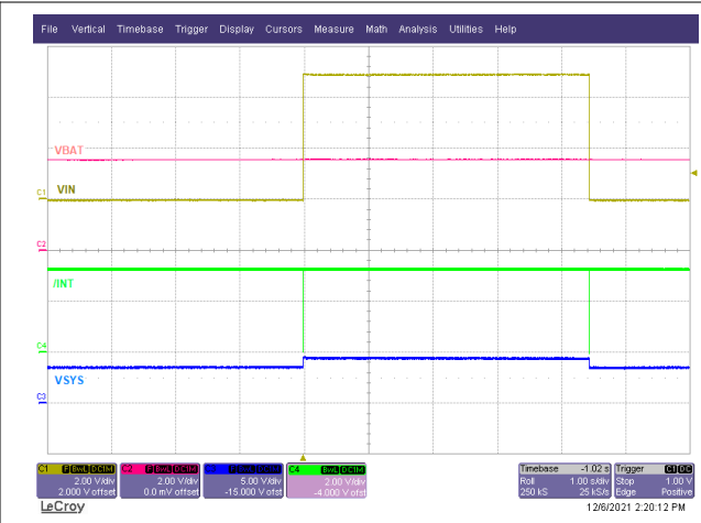
Figure 9-11. Power Good Interrupt on /INT
