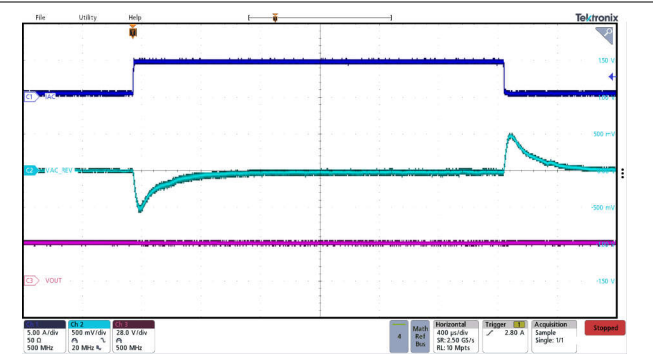
Figure 9-16. Reverse Mode Buck-Boost Transient Reponse
