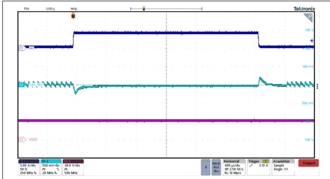
Figure 9-15. Reverse Mode Buck Transient Reponse
