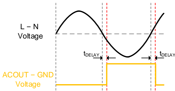
Figure 9. Zero Cross Delay Time (BM1Z002FJ)
