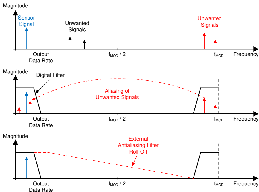
Figure 10-3. Effect of Aliasing
