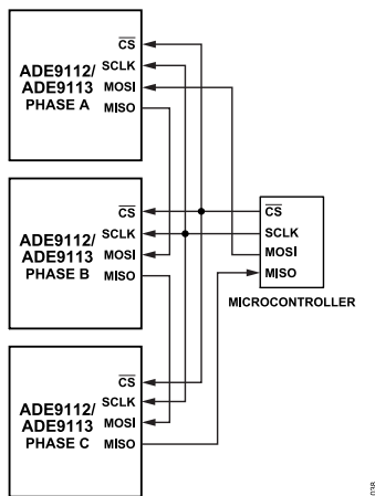
Figure 38. SPI Connection Between Three ADE9103/ADE9112/ADE9113 Devices in a Daisy Chain and a Microcontroller
