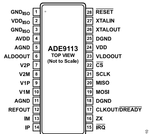
Figure 10. ADE9113 Pin Configuration
