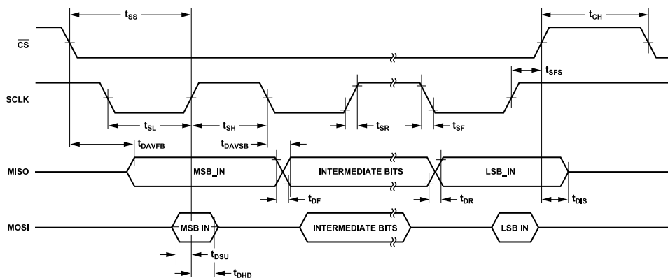
Figure 5. SPI Timing, CPOL = 1 and CHPA = 1
