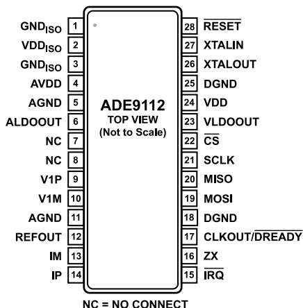
Figure 9. ADE9112 Pin Configuration
