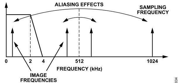
Figure 34. Aliasing Effects
