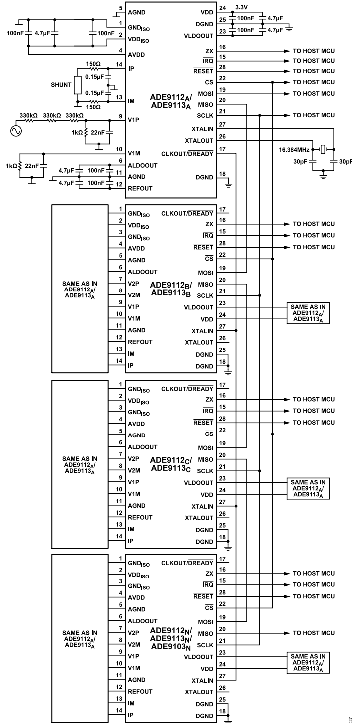
Figure 27. Test Circuit
