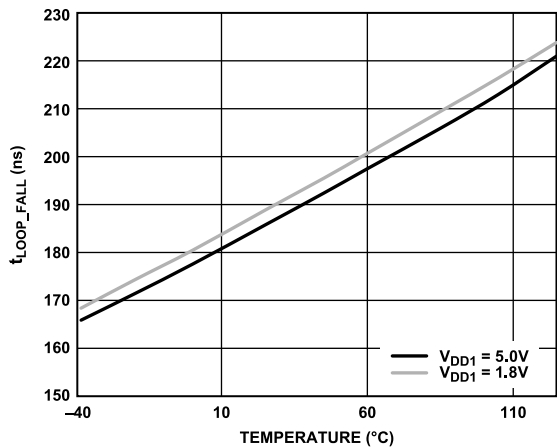
Figure 16. t_{LOOP\_FALL} vs. Temperature ( R_{SLOPE} = 47 k\Omega )
