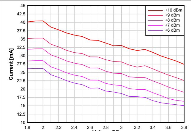
Figure 8-13. TX Current vs. Supply Voltage (VDD5) (BLE 1 Mbps, 2.44 GHz, +10 dBm PA)
