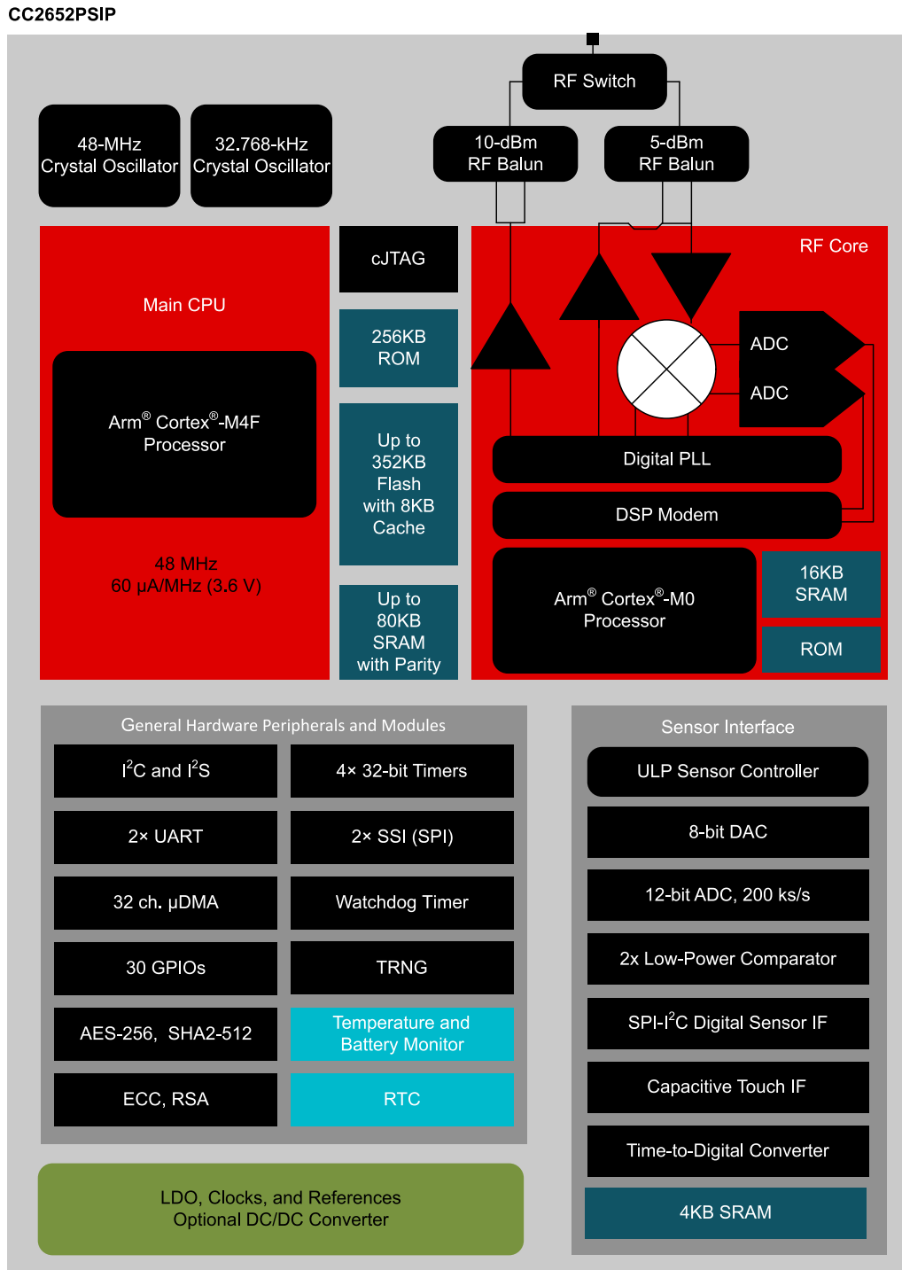
Figure 4-2. CC2652PSIP Hardware Overview
