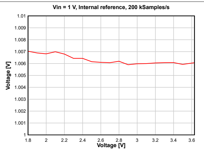
Figure 8-35. ADC Accuracy vs. Supply Voltage (VDD5)
