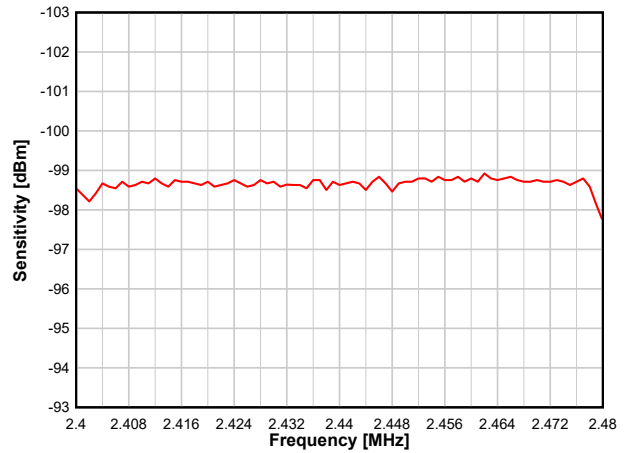
Figure 8-15. Sensitivity vs. Frequency (250 kbps)
