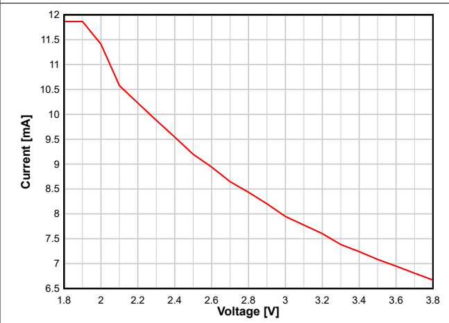
Figure 8-11. TX Current vs. Supply Voltage (VDD5) (BLE 1 Mbps, 2.44 GHz, 0 dBm)
