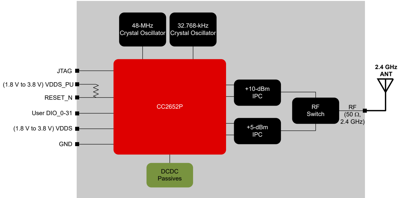
Figure 4-1. CC2652PSIP Block Diagram
