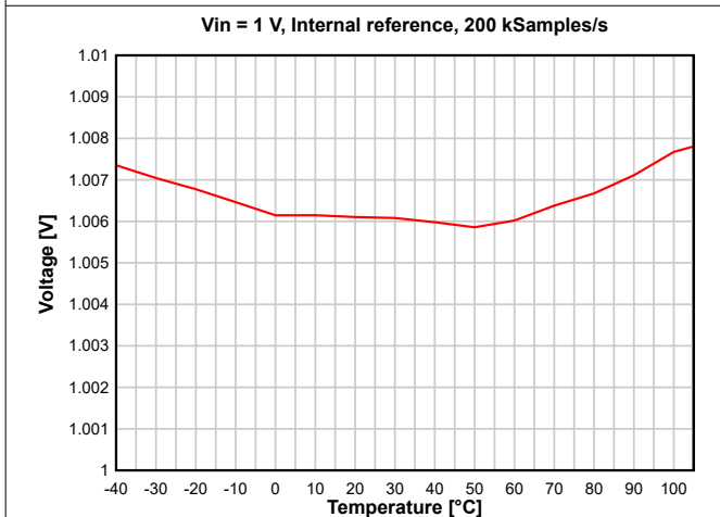
Figure 8-34. ADC Accuracy vs. Temperature
