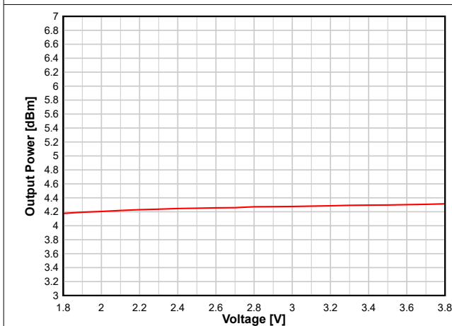
Figure 8-25. Output Power vs. Supply Voltage (VDD5) (BLE 1 Mbps, 2.44 GHz, +5 dBm)
