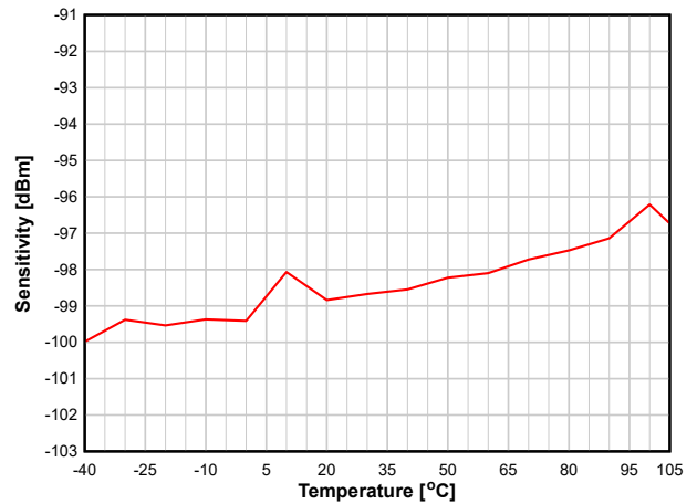
Figure 8-17. Sensitivity vs. Temperature (250 kbps, 2.44 GHz)
