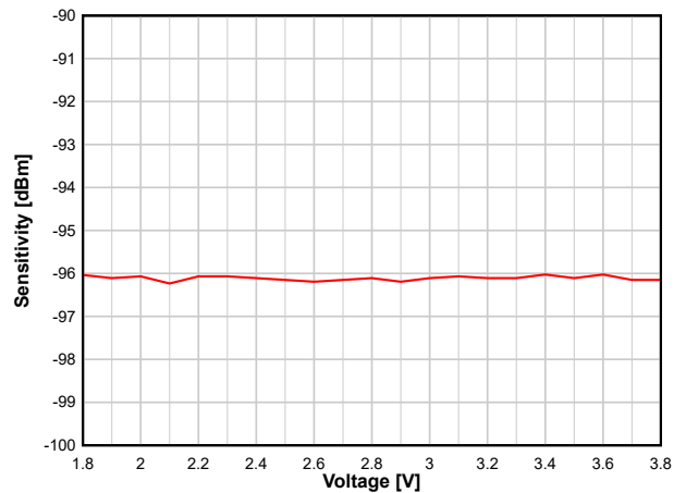
Figure 8-19. Sensitivity vs. Supply Voltage (VDD) (BLE 1 Mbps, 2.44 GHz, DCDC Off)
