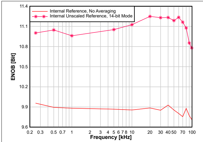
Figure 8-30. ENOB vs. Input Frequency
