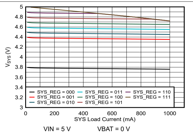
Figure 7-4. SYS Load Regulation
