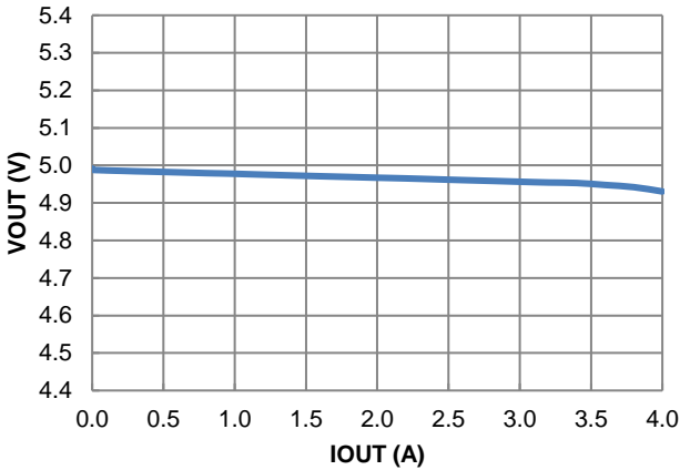
Figure 27. Load Regulation
