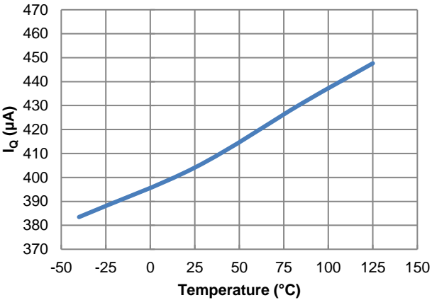
Figure 28. I_Q vs. Temperature
