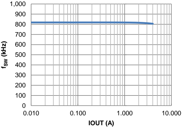
Figure 30. f_{sw} vs. Load
