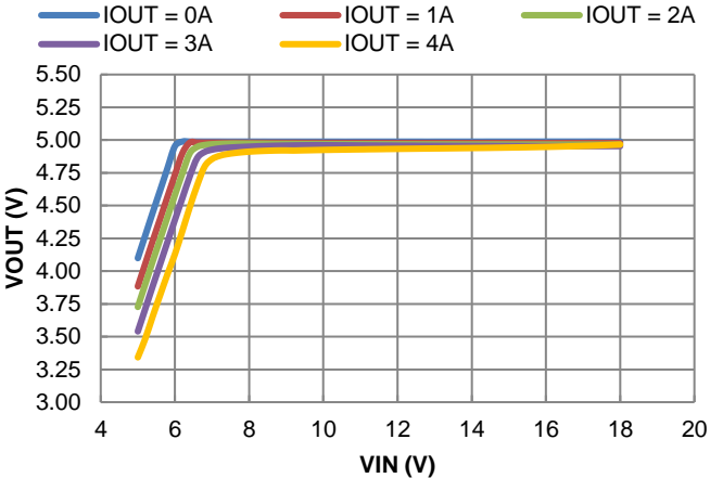
Figure 26. Line Regulation
