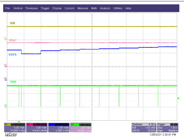
Figure 9-13. SYS Regulation Sweep
