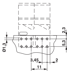
Drilling diagram
