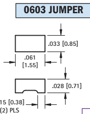
Mounting Detail
