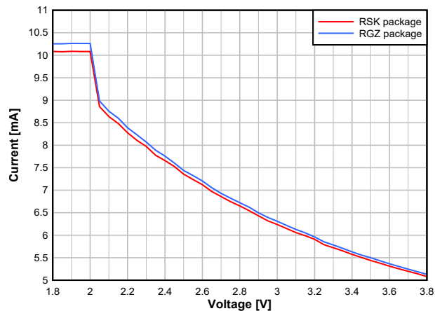
Figure 7-8. RX Current vs. Supply Voltage (VDDS) (50kbps, 868.3MHz)
