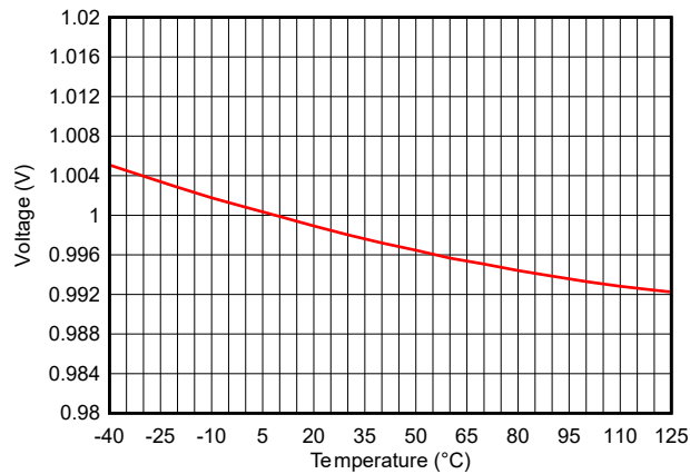
Figure 7-34. ADC Accuracy vs Temperature ( V_{in} =1V, Internal Reference, 200ksps)
