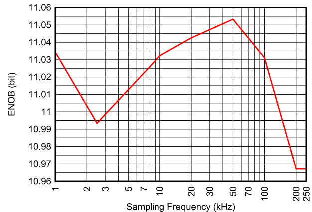
Figure 7-29. ENOB vs Sampling Frequency ( V_{in}=3V Ramp Wave, Internal Reference, F_{in}=F_s/10 )
