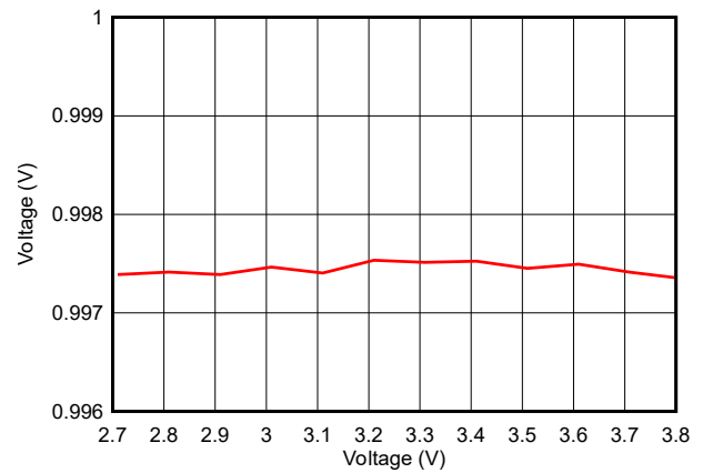
Figure 7-35. ADC Accuracy vs Supply Voltage ( V_{in} =1V, Internal Reference, 200ksps)
