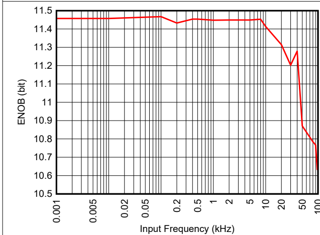
Figure 7-30. ENOB vs Input Frequency (External Reference = 3.0V)
