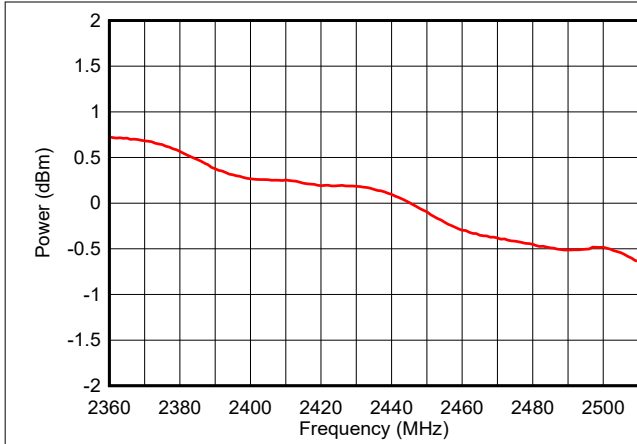
Figure 7-26. Output Power vs Frequency (BLE 1Mbps, 0dBm)
