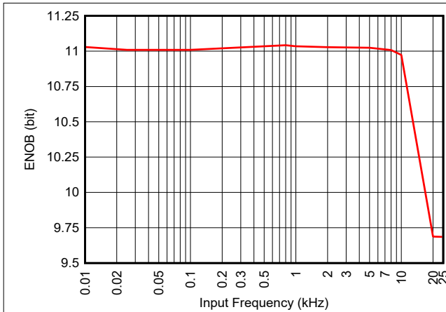
Figure 7-28. ENOB vs Input Frequency (Internal Reference)
