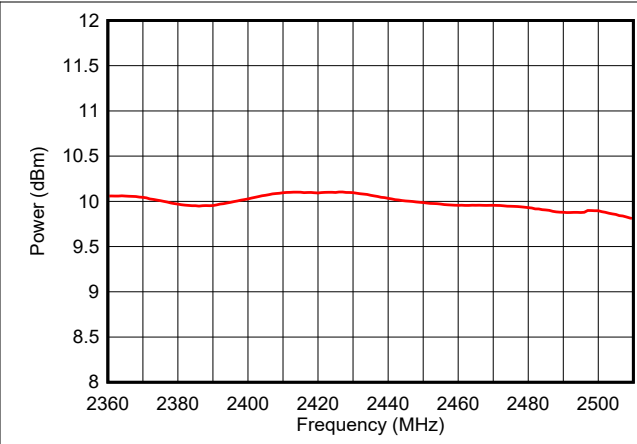
Figure 7-27. Output Power vs Frequency (BLE 1Mbps, +10dBm)
