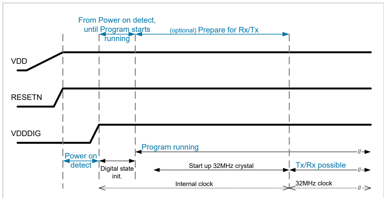
Figure 14: Power On Timing (not to scale)
