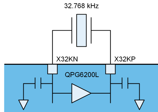
Figure 17: 32 KiHz Crystal Configuration
