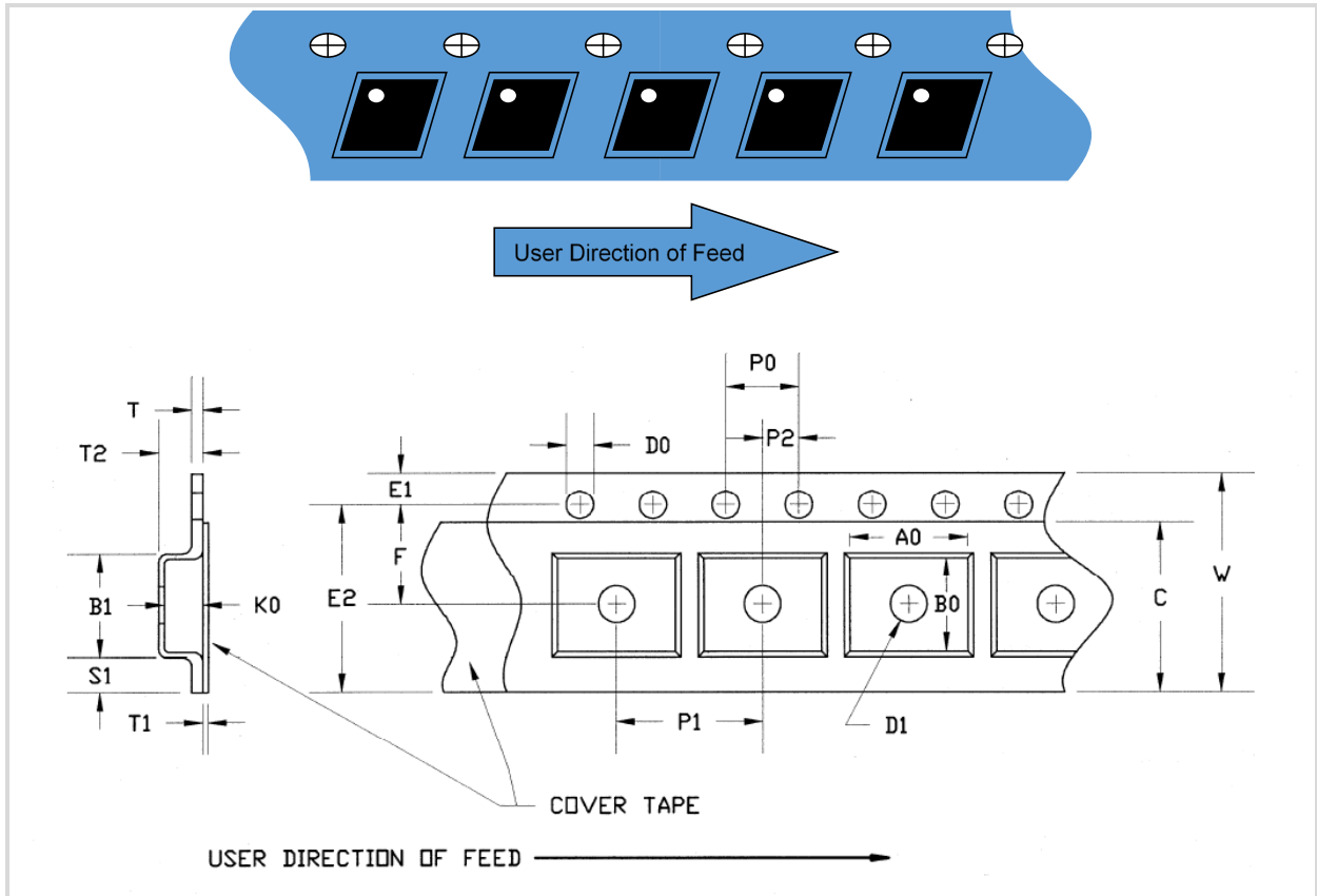
Figure 23: Carrier and Cover Tape Dimensions
