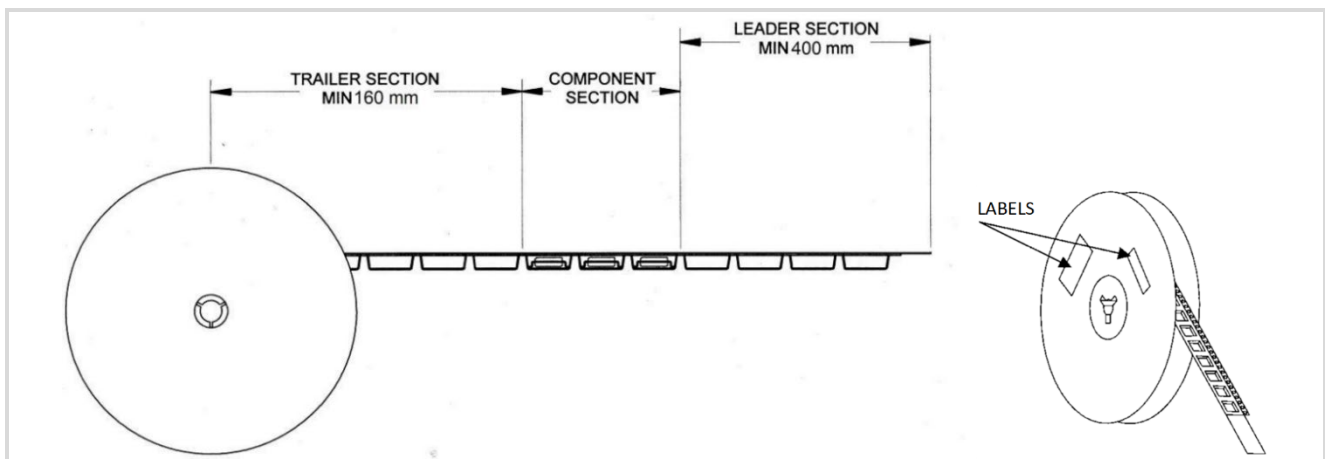
Figure 25: Tape and Labels
