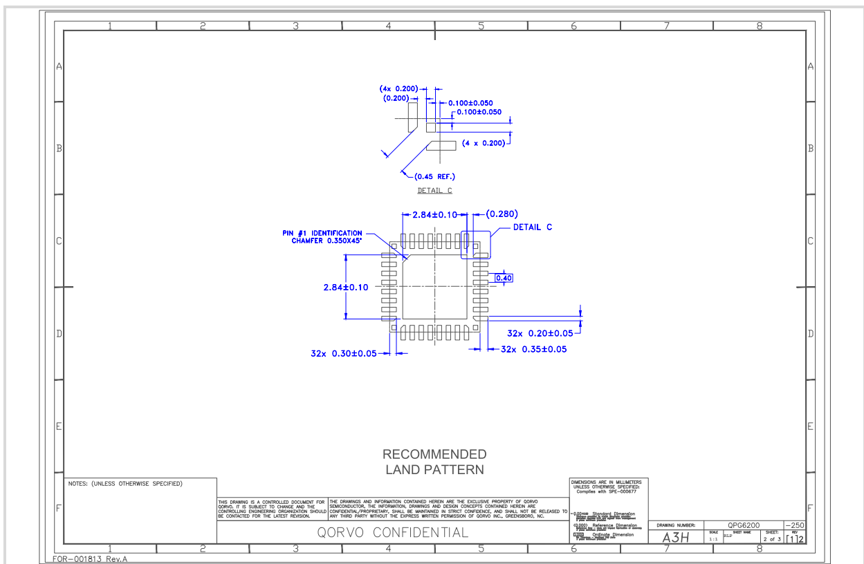
Figure 21: Recommended Land Pattern
