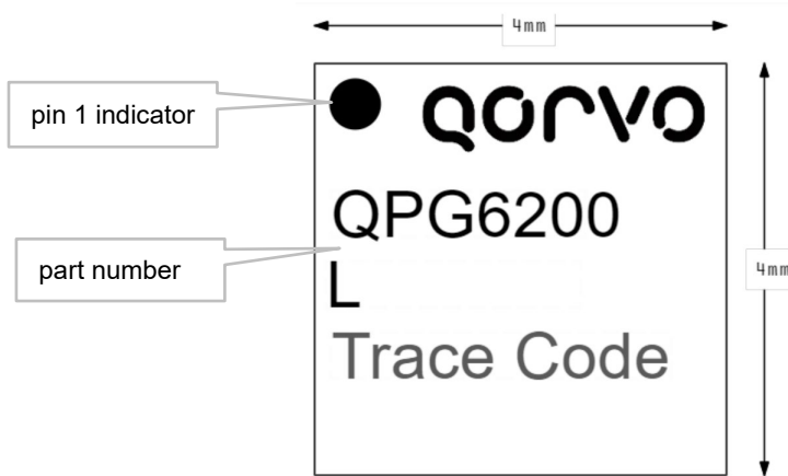
Figure 22: Package Information
