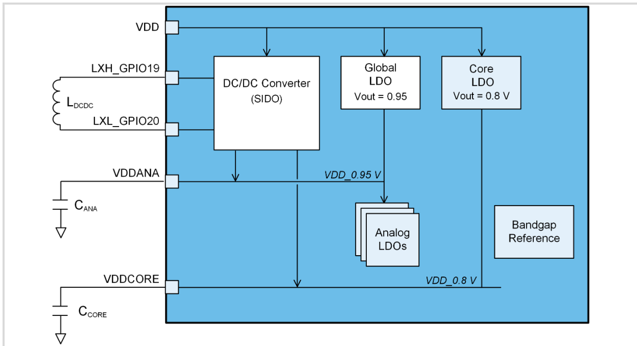
Figure 8: DC/DC Converter
