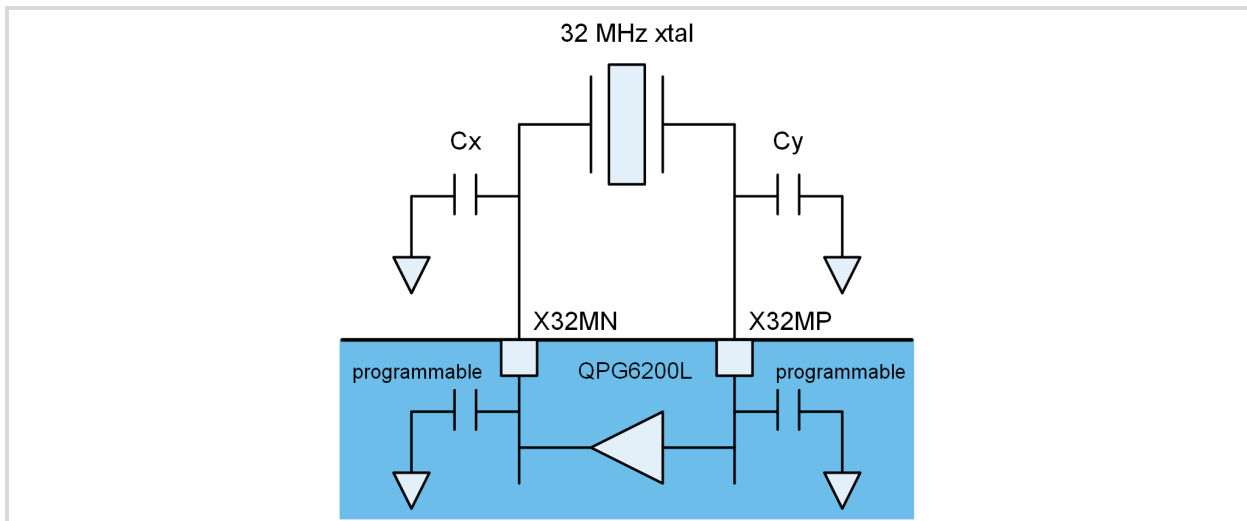
Figure 16: Typical 32 MHz Crystal Configuration
