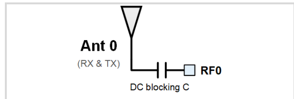
Figure 1: Single Antenna
