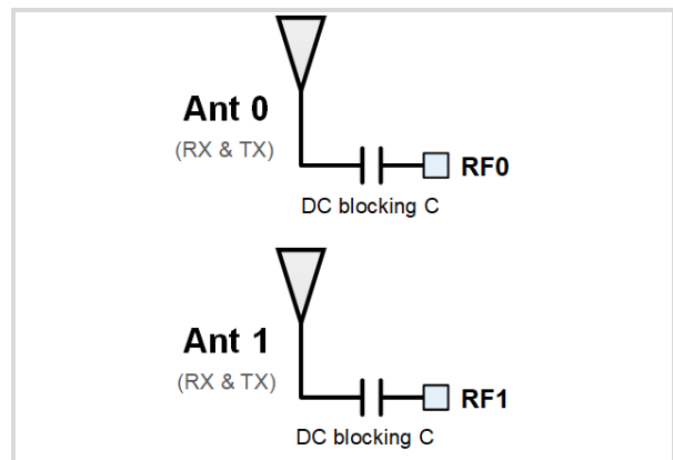
Figure 2: Two Antennas
