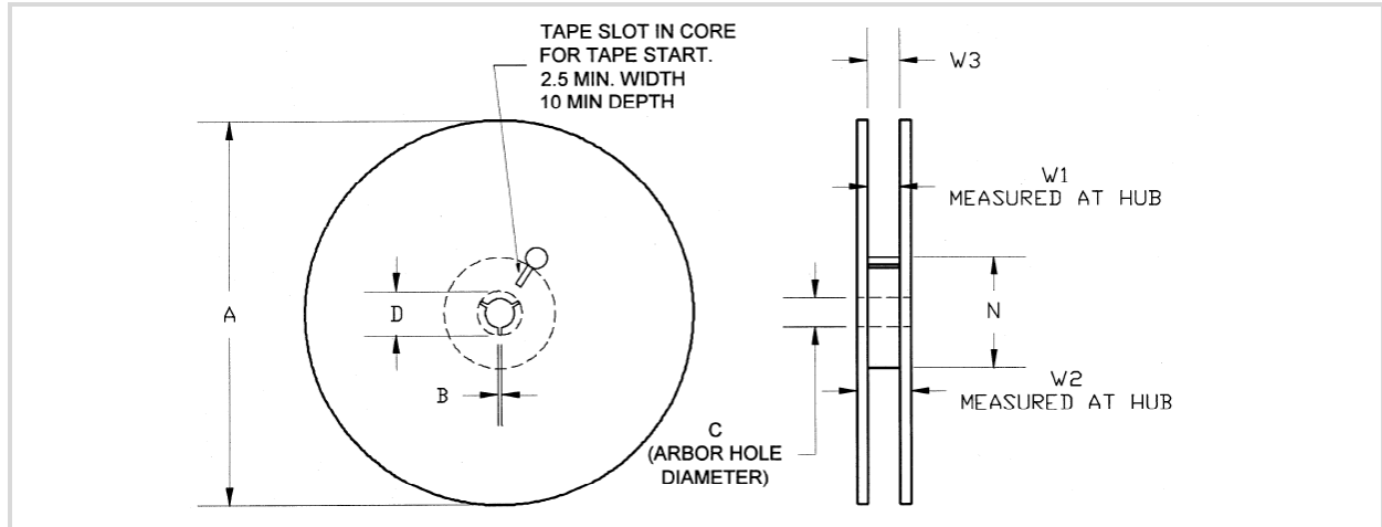
Figure 24: Reel Dimensions
