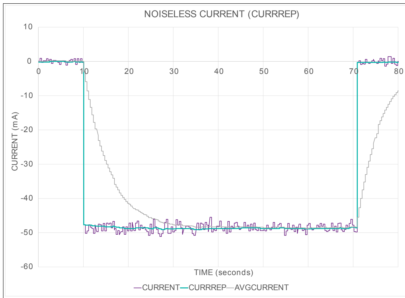
Figure 27. Noiseless Current
