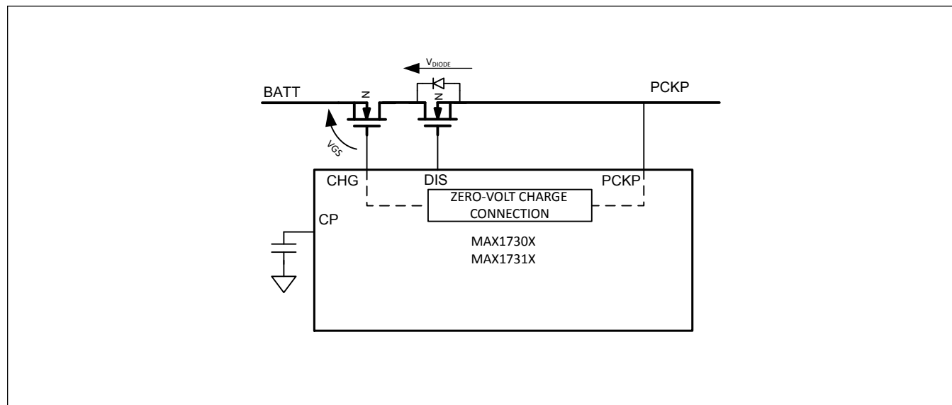
Figure 9. Zero-Volt Charging Diagram
