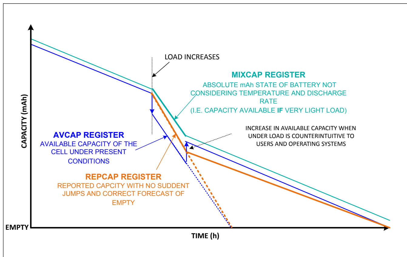
Figure 16. Handling Changes in Empty Calculation
