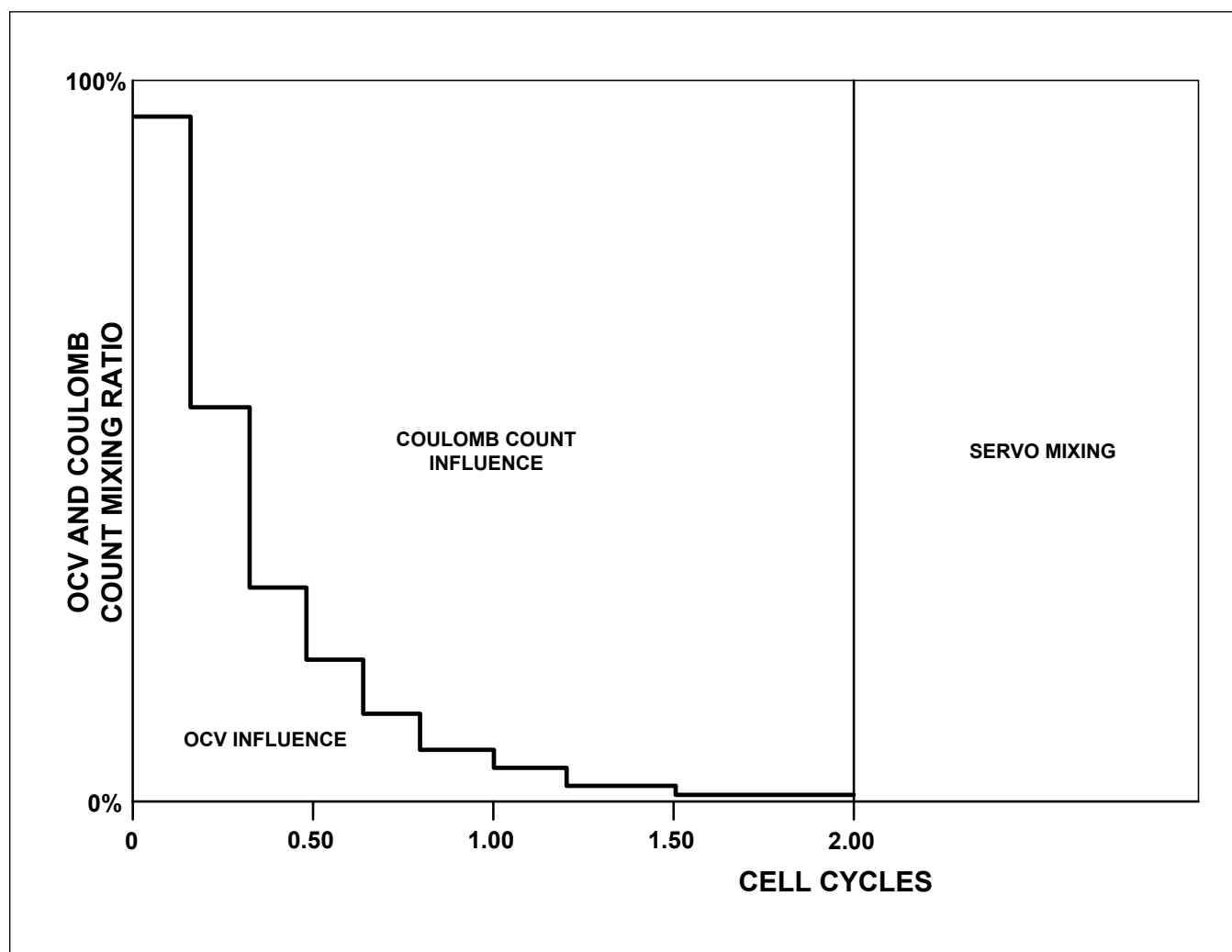
Figure 14. Voltage and Coulomb Count Mixing
