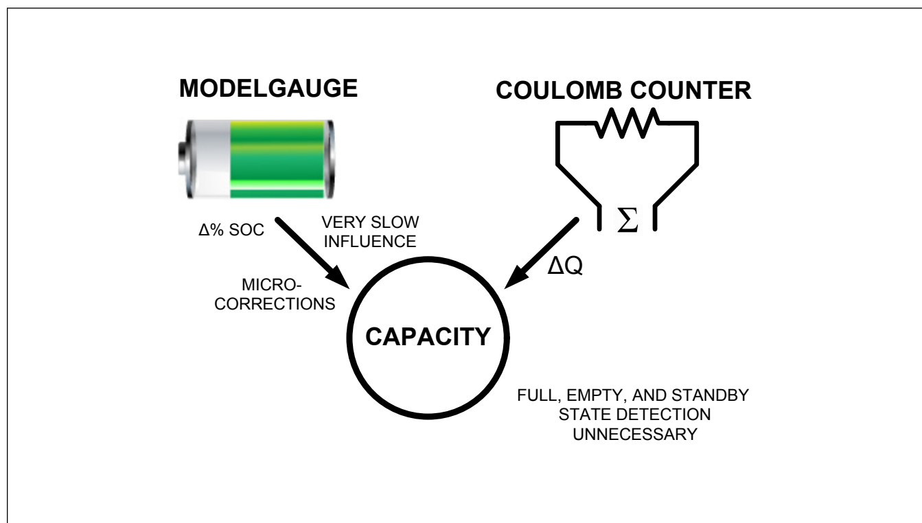
Figure 10. Merger of Coulomb Counter and Voltage Based Fuel Gauge
