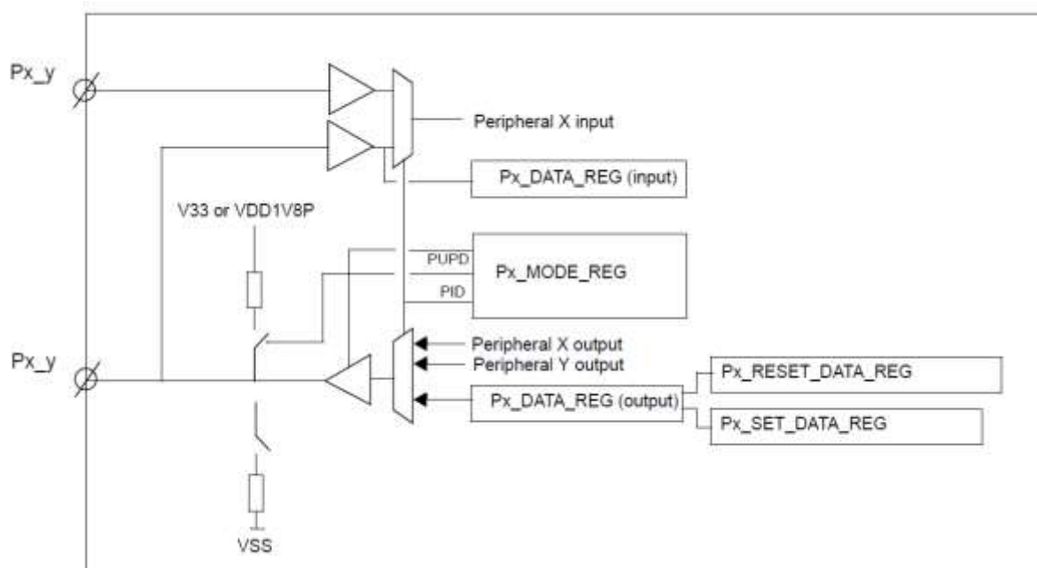
Figure 108. Port P0 and P1 with Programmable Pin Assignment
