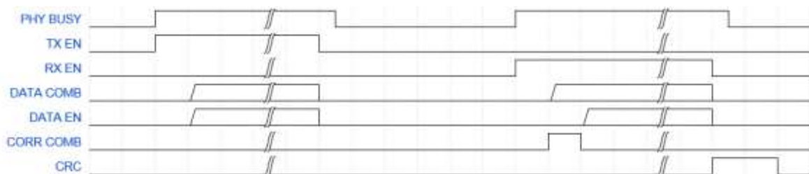
Figure 32. CMAC diagnostics timing diagram
