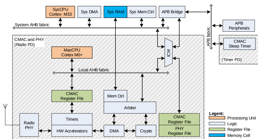
Figure 31. Configurable MAC block diagram
