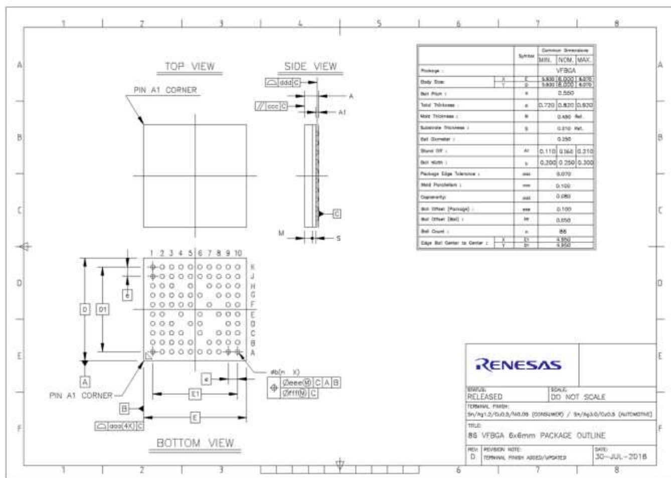
Figure 112. VFBGA86 Package outline drawing
