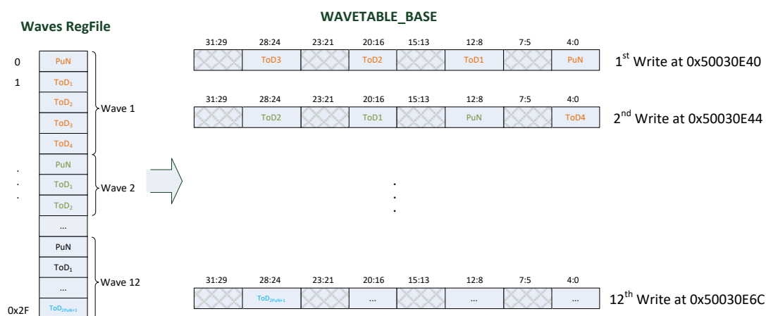
Figure 50. Loading waves into waves memory space
