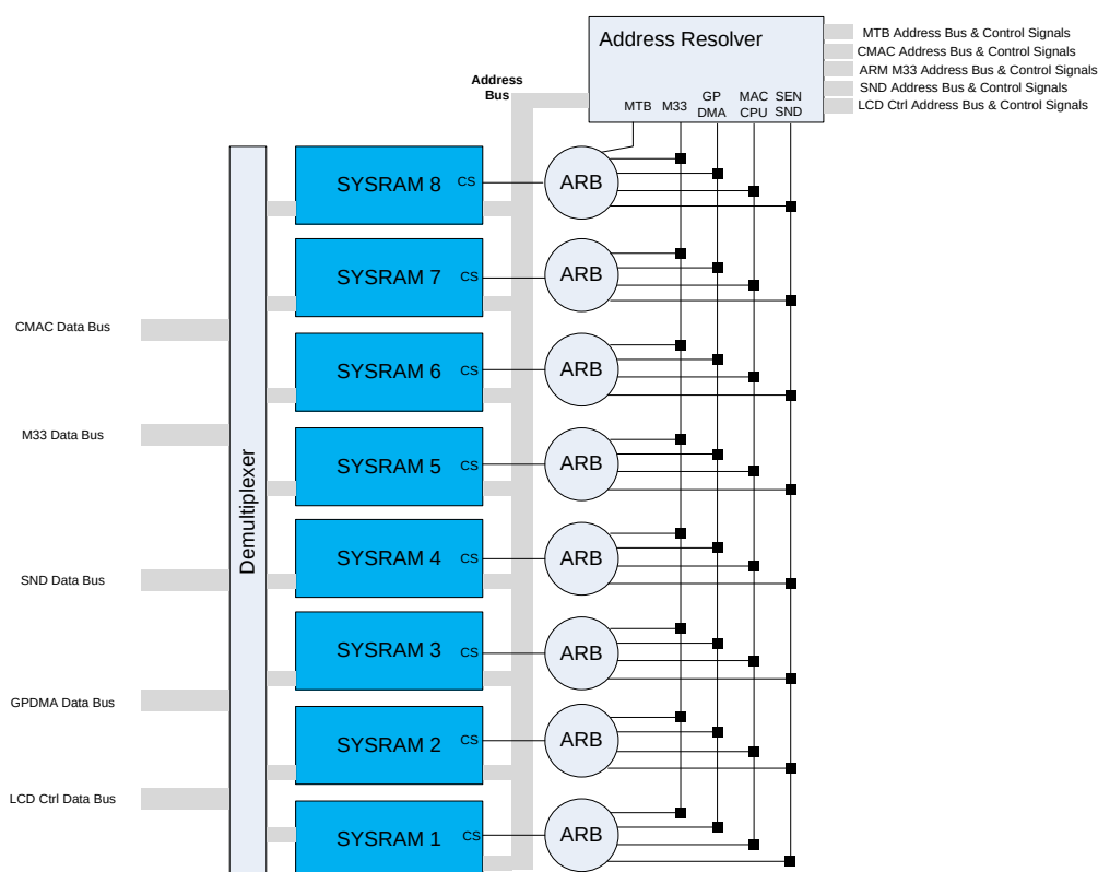
Figure 34. Internal architecture of the memory controller
