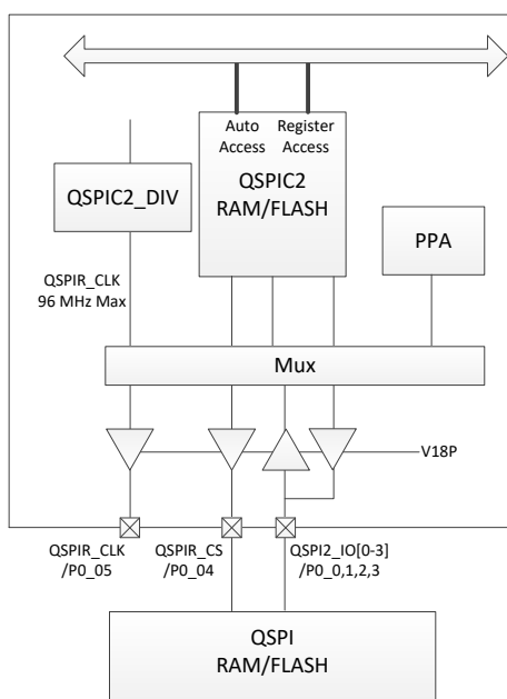
Figure 44. Quad SPI RAM/Flash controller
