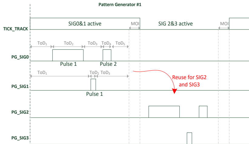
Figure 51. Waveform generation in signal pairs
