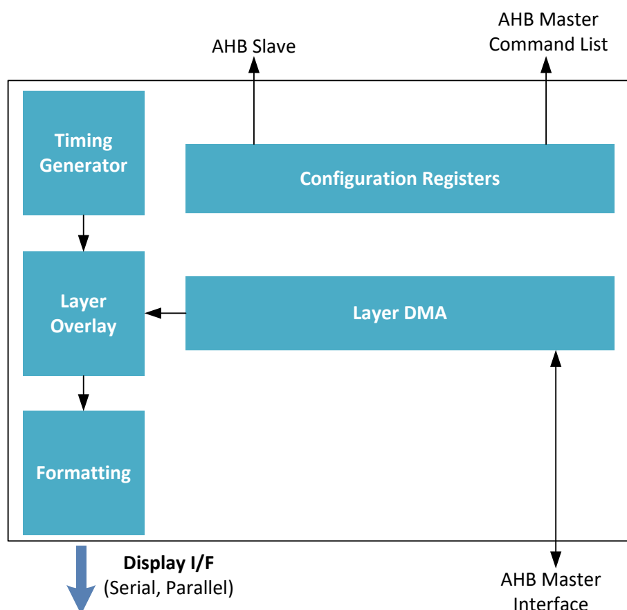
Figure 52. LCD controller block diagram
