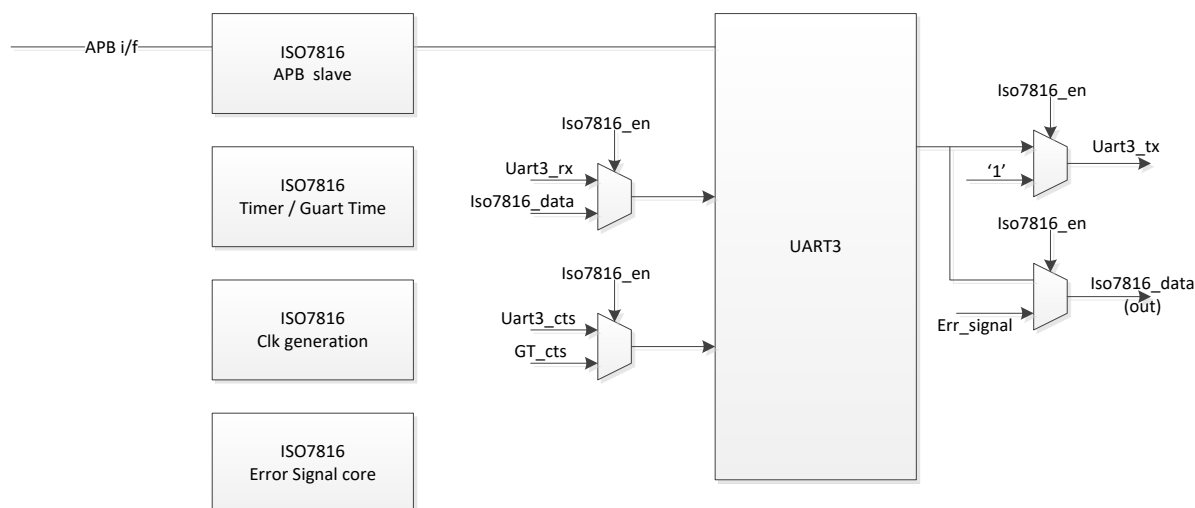
Figure 85. Smart Card (ISO7816-3) block diagram
