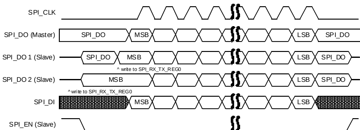
Figure 87. SPI Master/Slave mode 0: SPI_POL=0 and SPI_PHA=0
