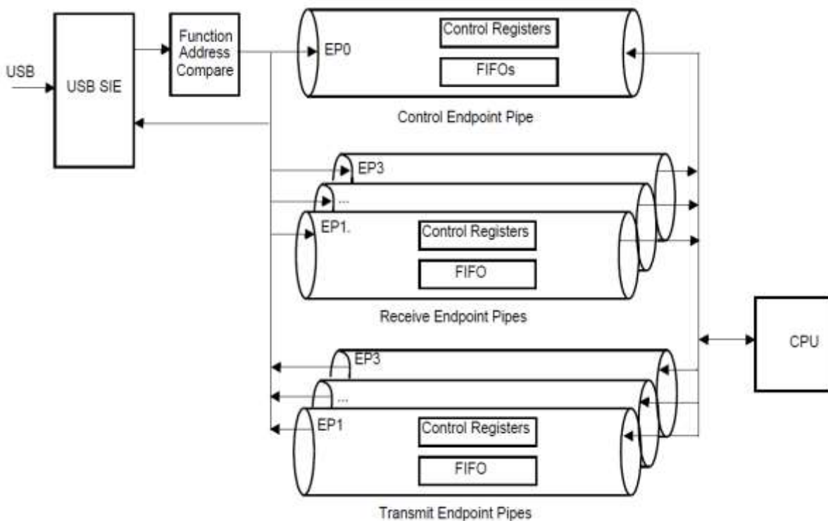
Figure 96. Endpoint operation
