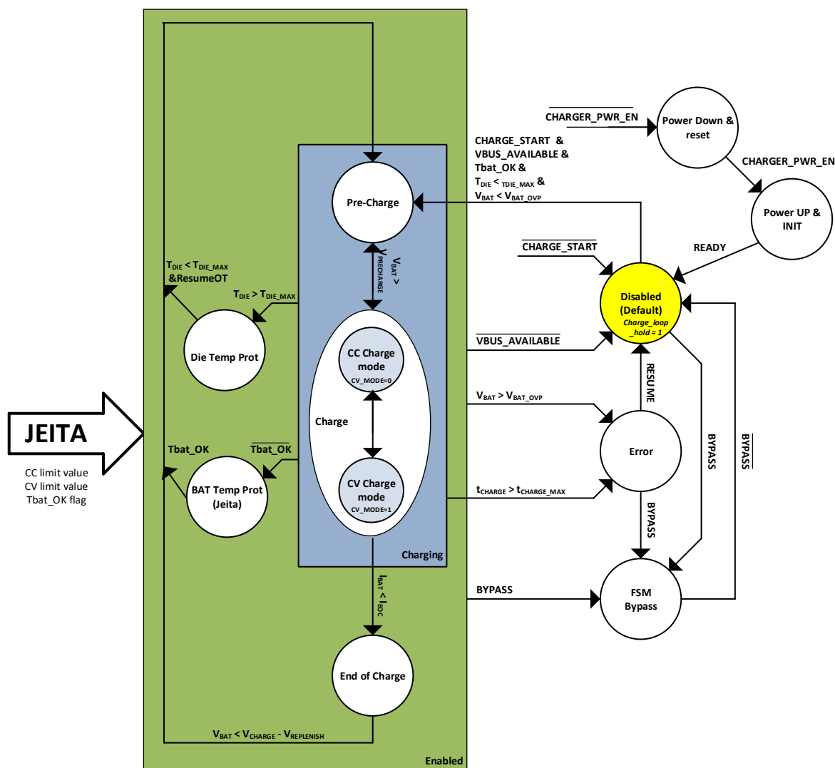
Figure 18. Charger hardware finite state machine diagram
