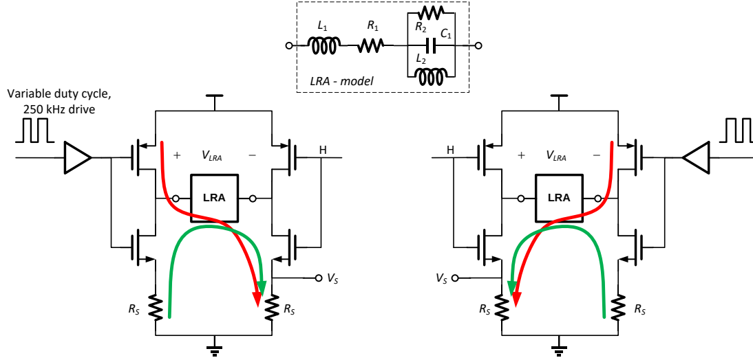
Figure 106. Circuit diagram of the Haptic Driver and Equivalent electrical model of an LRA
