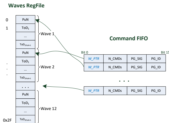
Figure 49. Commands and waveform format
