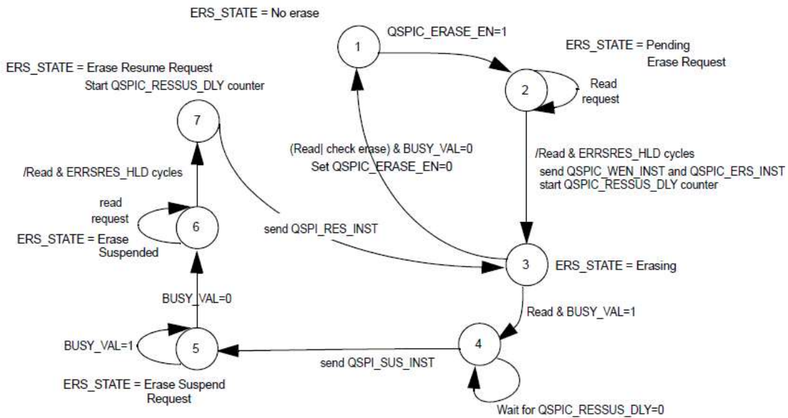
Figure 41. Erase suspend/resume in Auto mode
