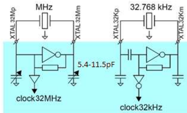
Figure 37. Crystal oscillator circuits
