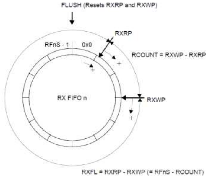
Figure 101. USB Rx FIFO operation
