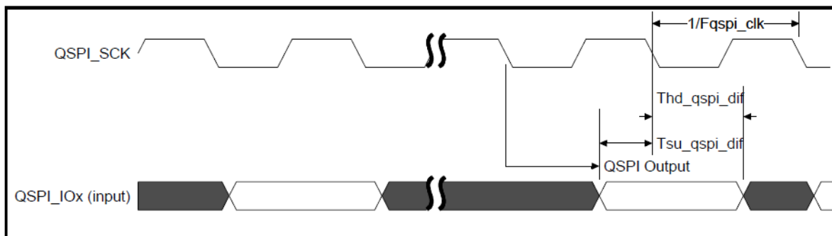
Figure 42: QSPI input timing
