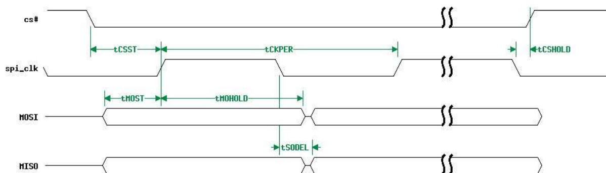
Figure 91. SPI Slave mode timing (CPOL = 0, CPHA = 0)
