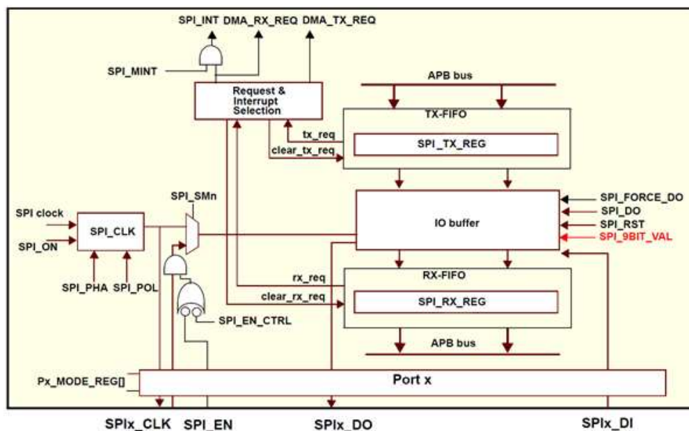
Figure 86. SPI block diagram
