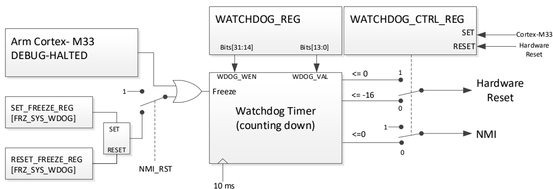
Figure 94. System watchdog block diagram
