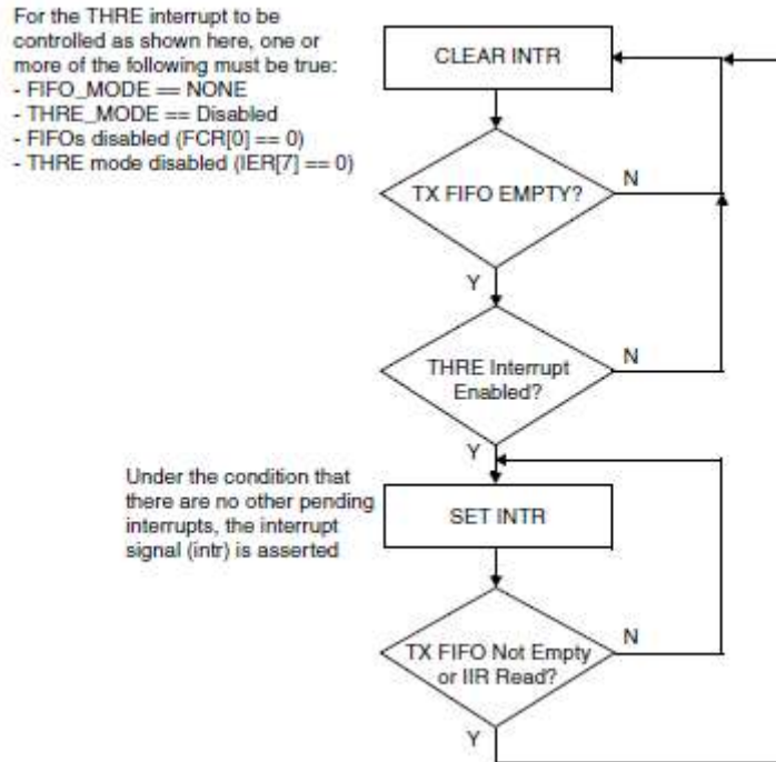
Figure 84. Flowchart of interrupt generation when not in programmable THRE Interrupt mode
