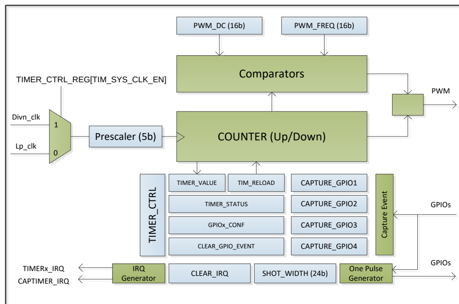
Figure 93. General Purpose Timer's block diagram
