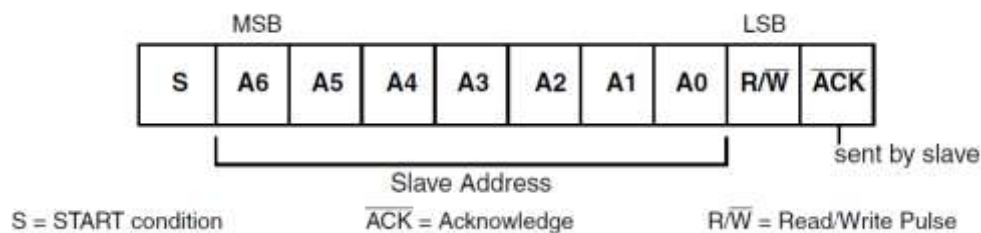
Figure 73. 7-bit address format
