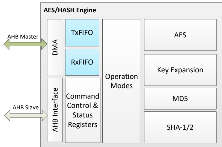
Figure 57. AES/HASH architecture
