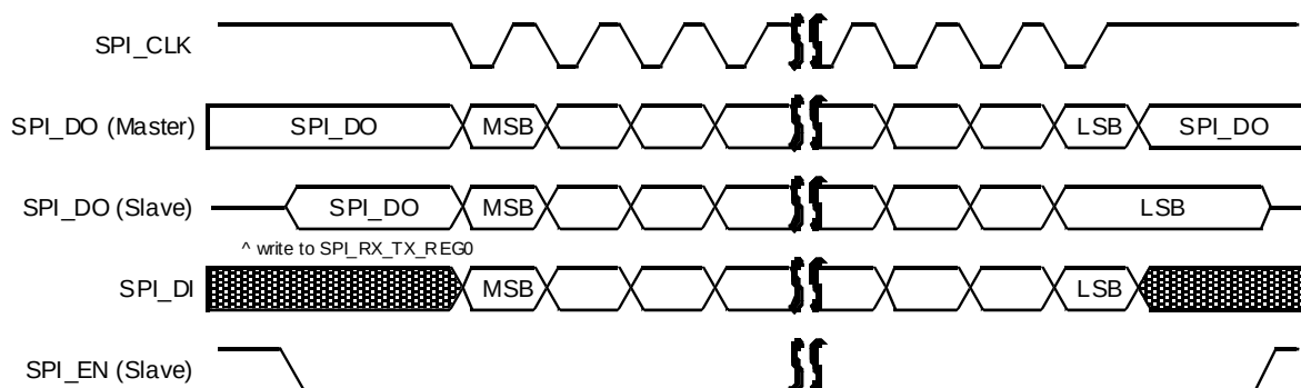
Figure 90. SPI Master/slave mode 3: SPI_POL=1 and SPI_PHA=1
