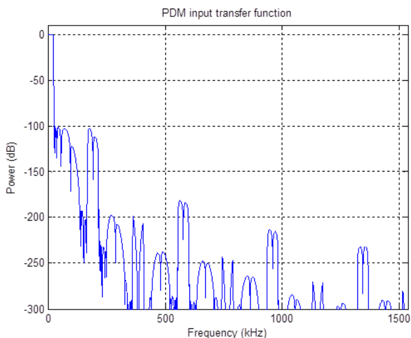
Figure 69. SRC PDM input transfer function
