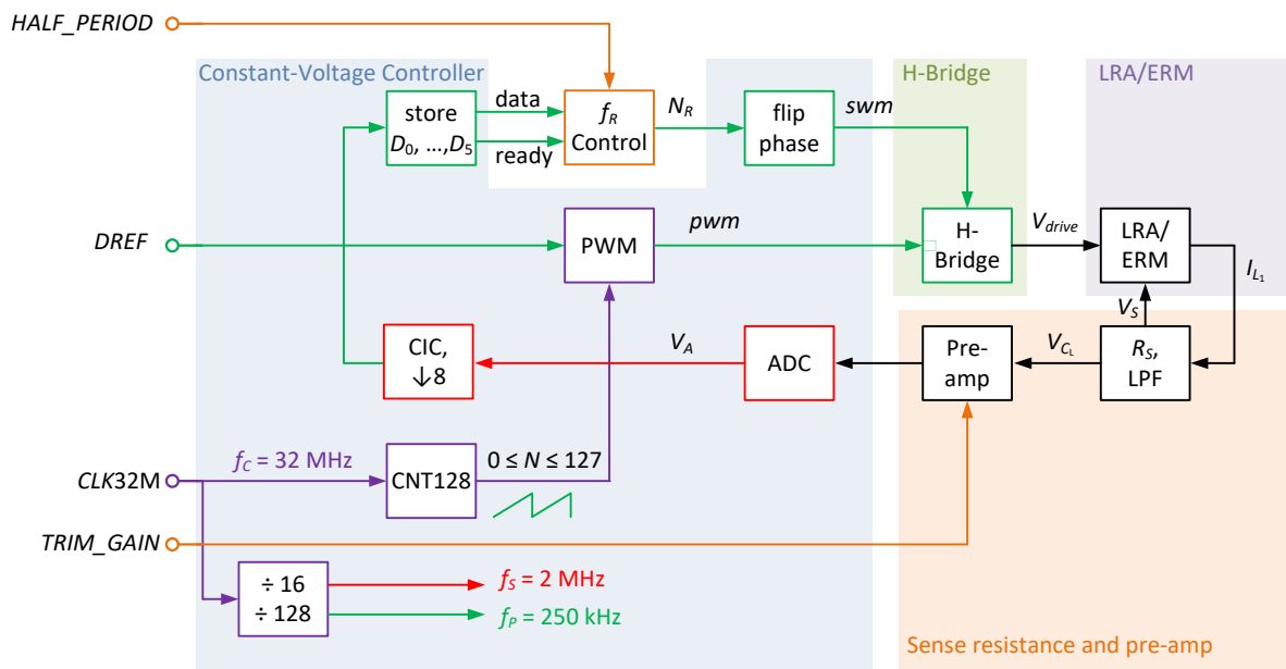
Figure 105. Block diagram of the haptic driver
