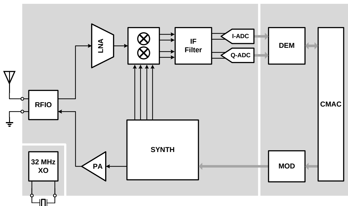
Figure 111. Radio block diagram
