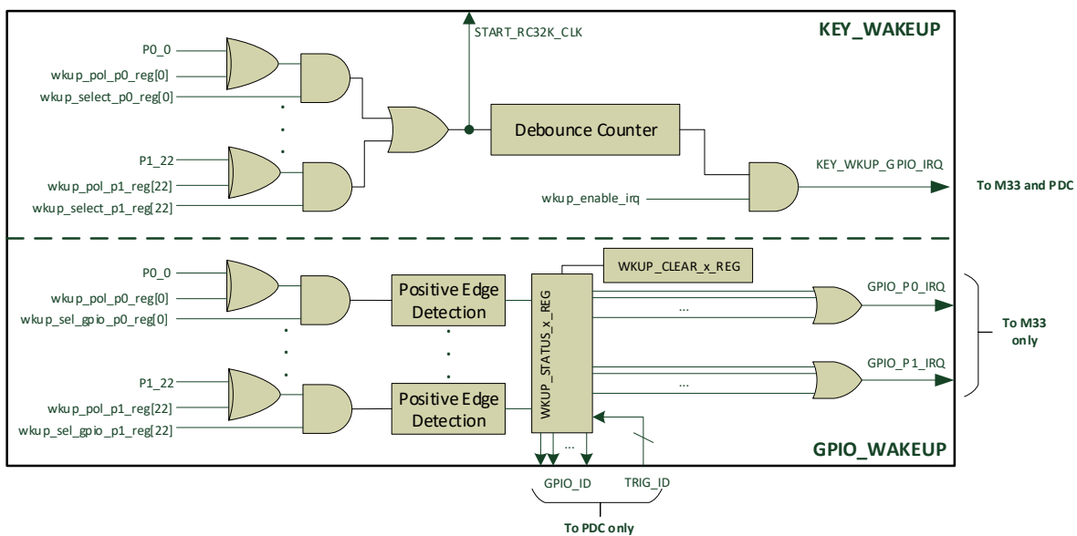
Figure 59: Wake-up controller block diagram
