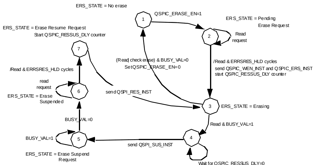
Figure 45. Erase suspend/resume in Auto mode
