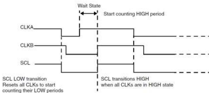
Figure 79. Multiple Master clock synchronization
