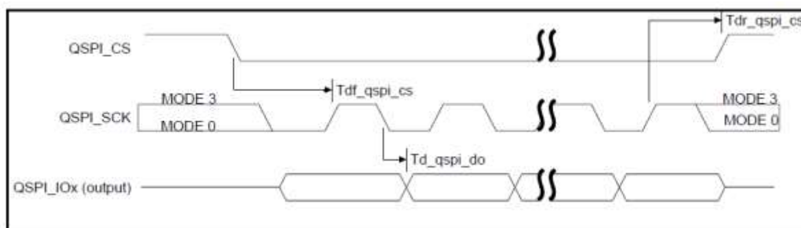
Figure 43: QSPI output timing
