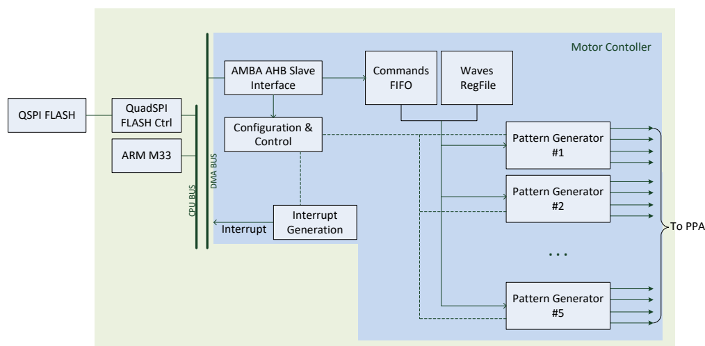
Figure 48. Motor Controller block diagram
