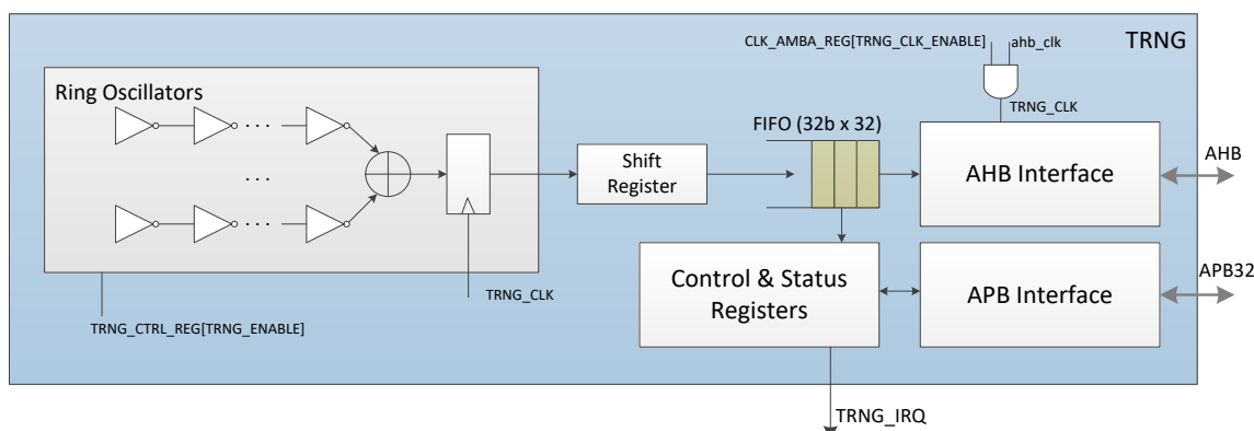
Figure 58. TRNG block diagram
