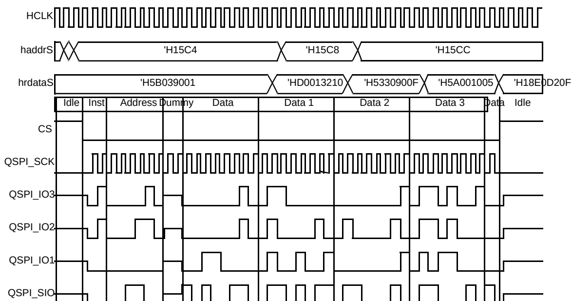
Figure 47. QSPI Burst timing for high performance (QSPI_FORENSEQ_EN=0)
