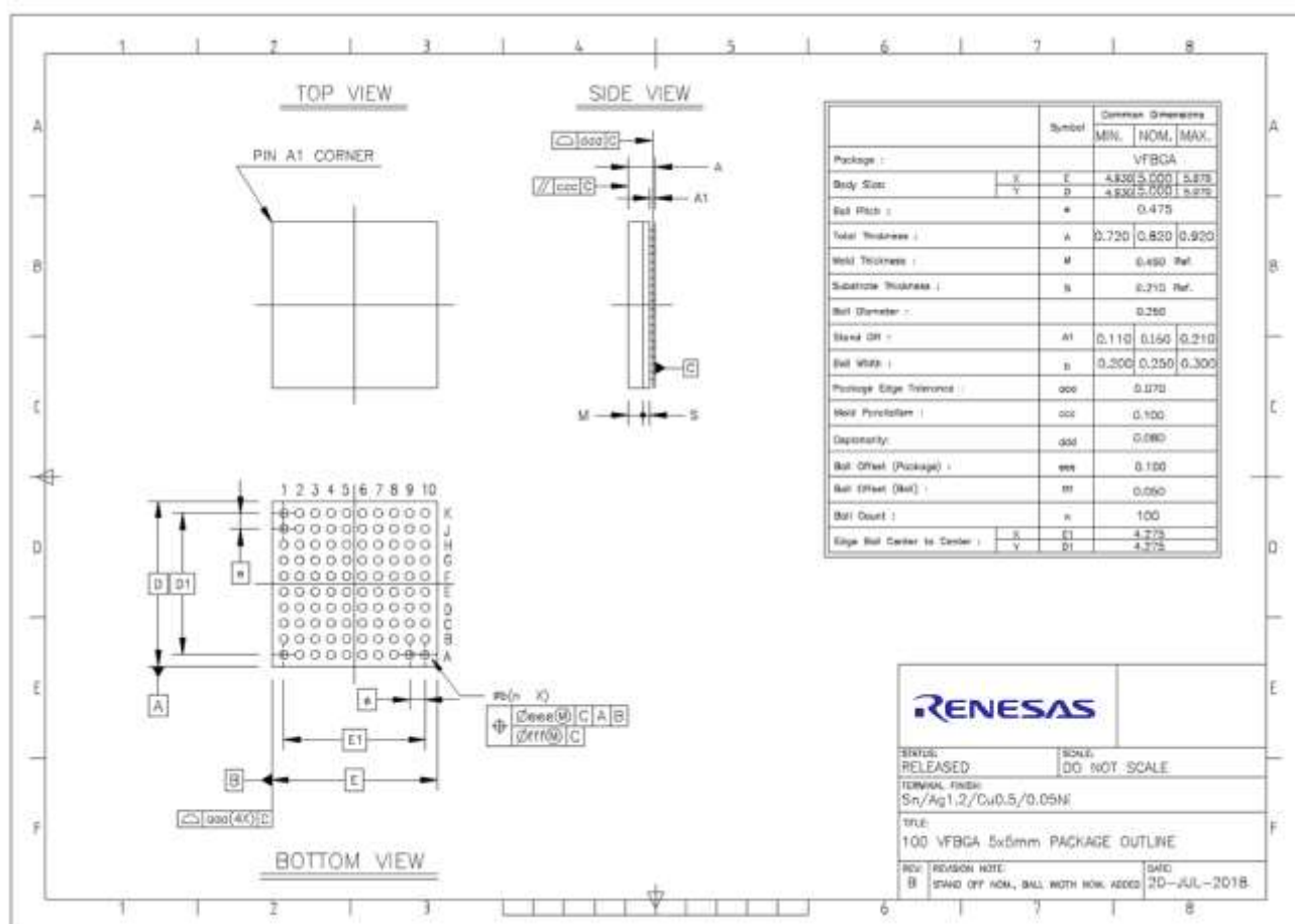
Figure 113. VFBGA100 Package outline drawing
