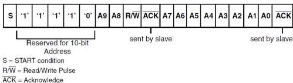
Figure 74. 10-bit address format
