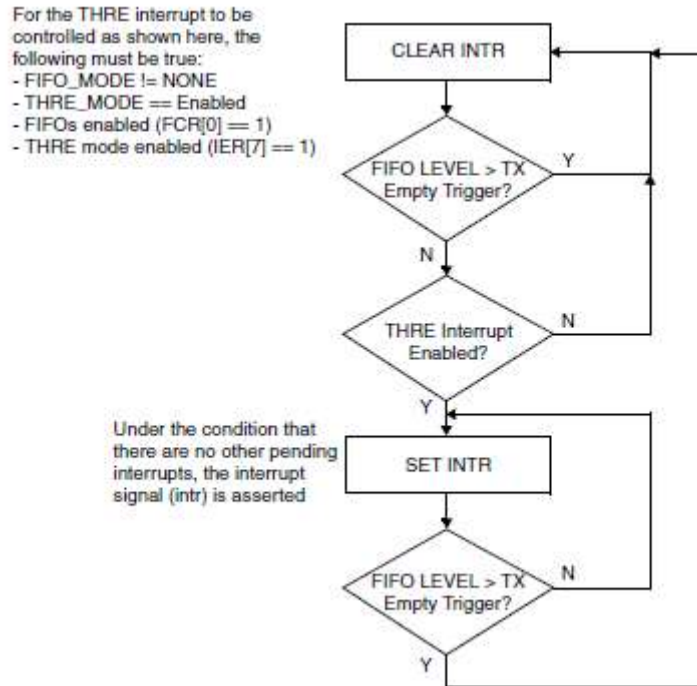
Figure 83. Flowchart of interrupt generation for programmable THRE Interrupt mode
