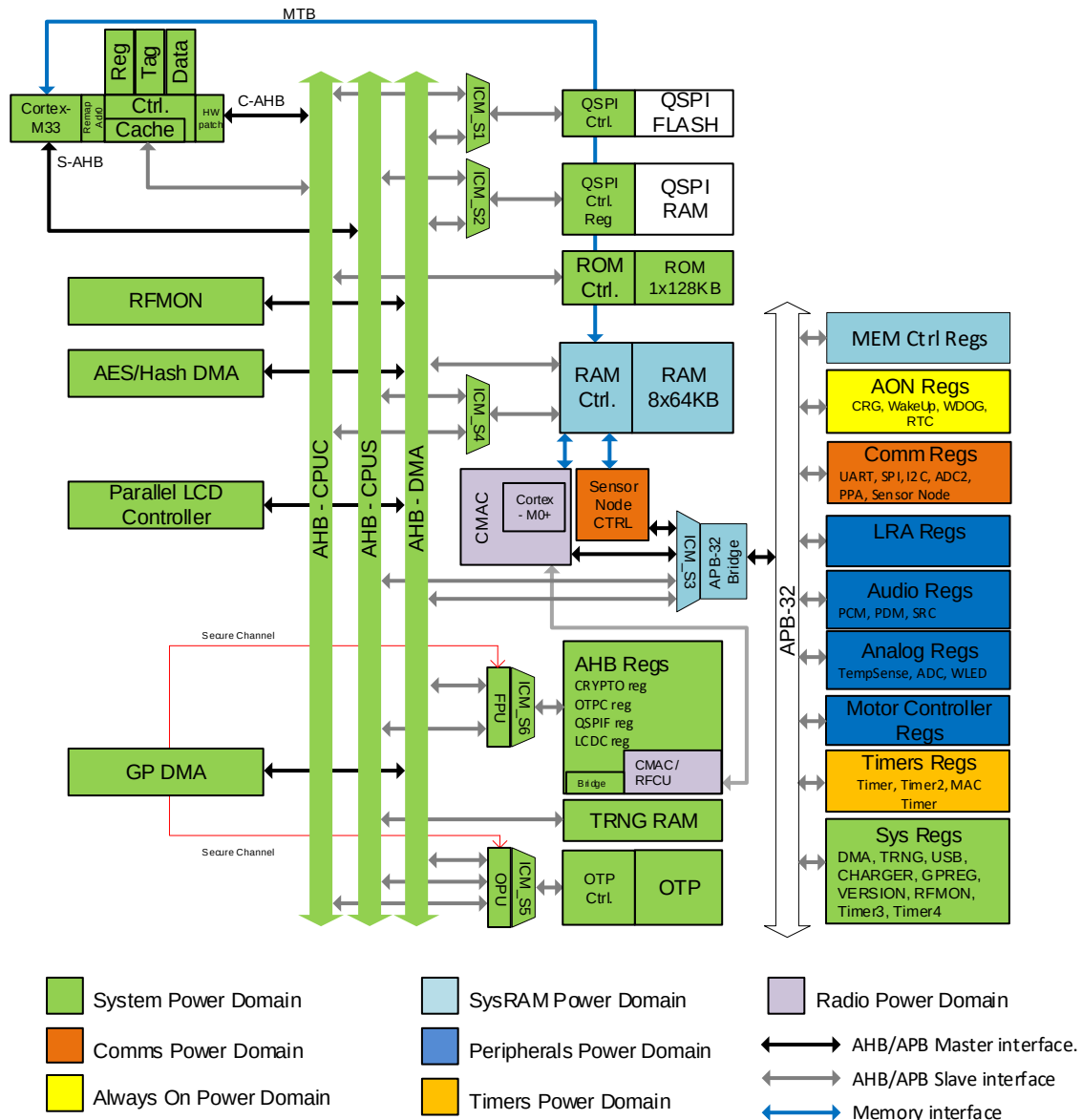
Figure 30. Bus architecture
