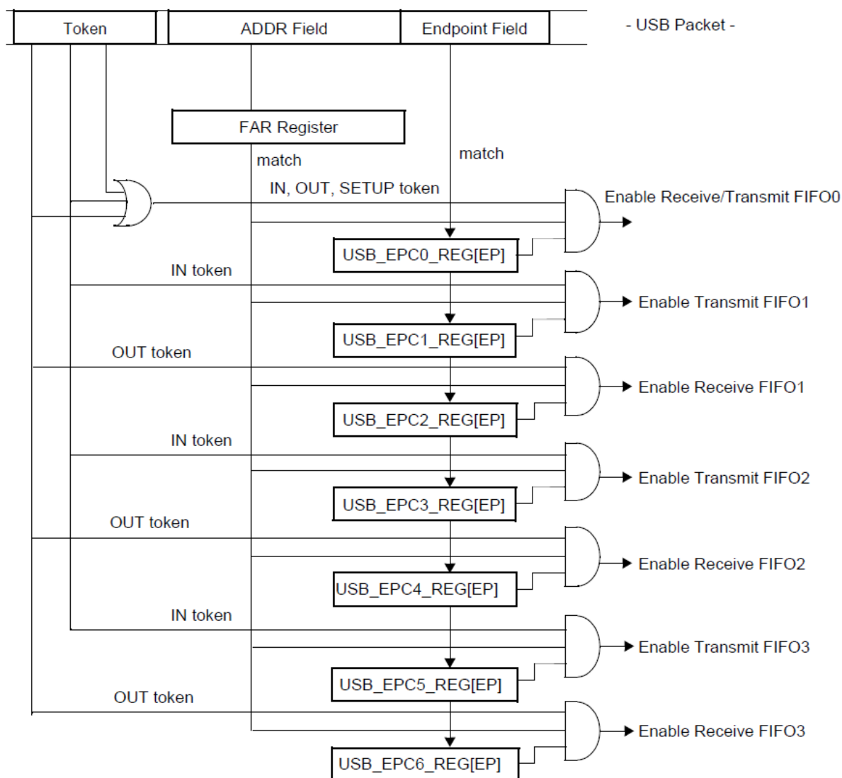
Figure 98. USB function address/endpoint decoding
