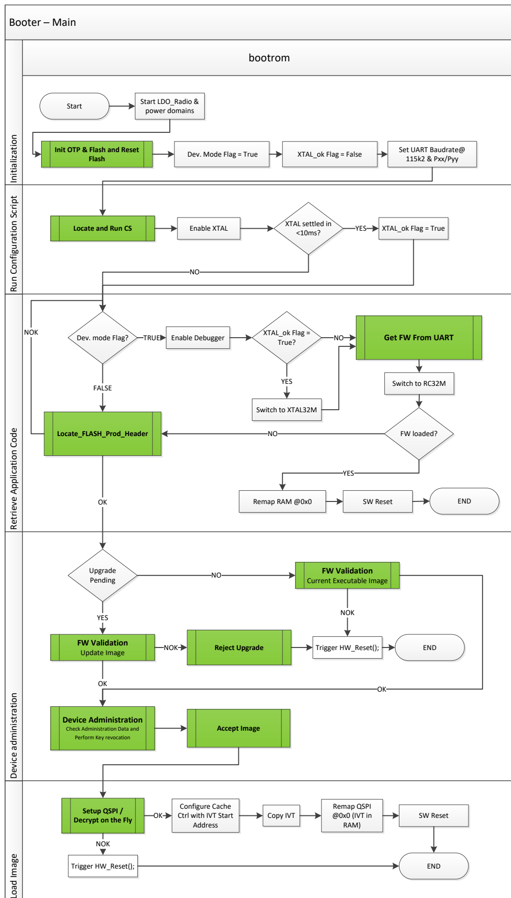
Figure 14. BootROM flowchart
