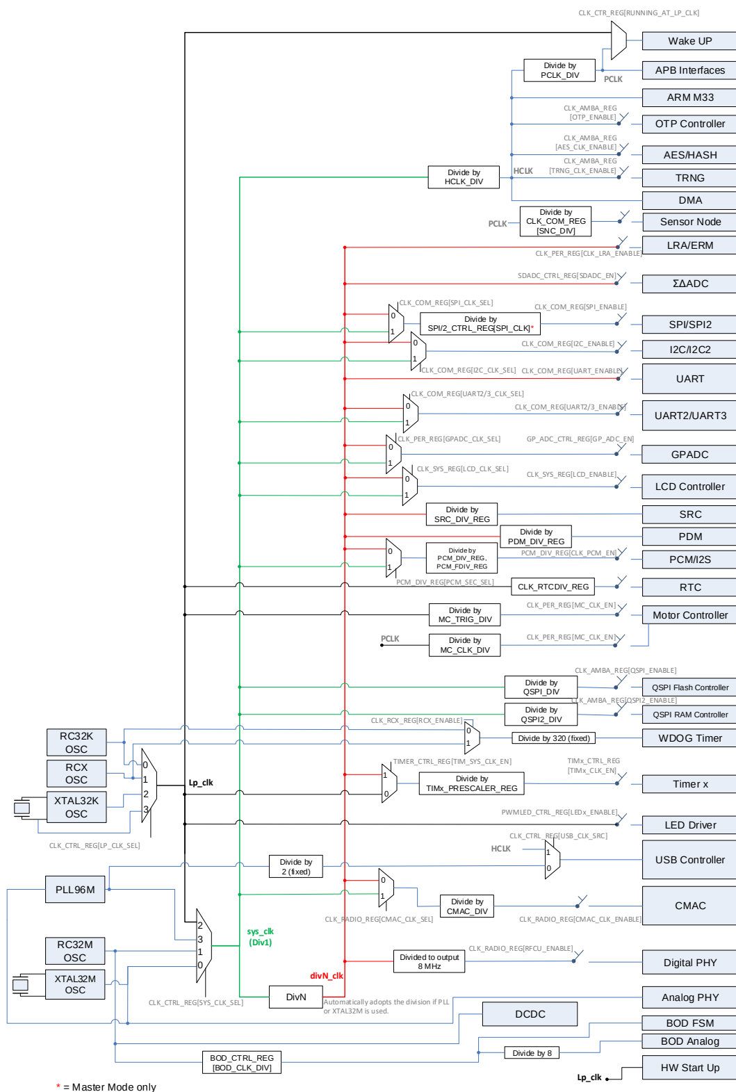
Figure 36. Clock tree diagram
