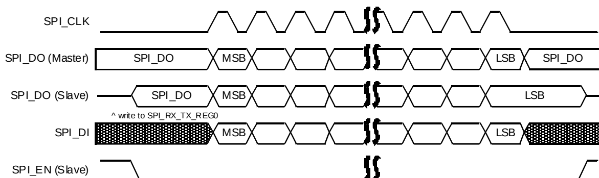
Figure 88. SPI Master/Slave mode 1: SPI_POL=0 and SPI_PHA=1
