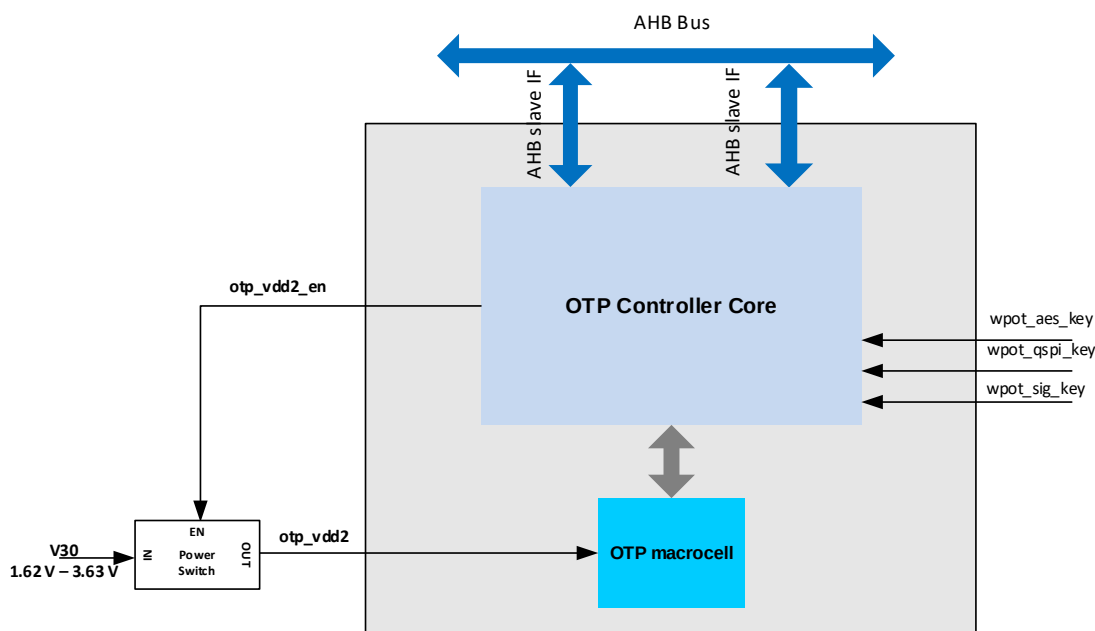
Figure 39. OTP controller block diagram
