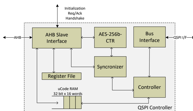
Figure 40. QSPI flash controller block diagram
