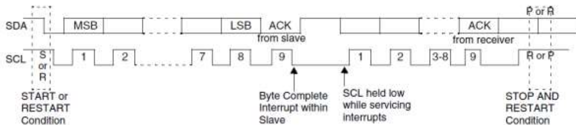
Figure 71. Data transfer on the I2C bus
