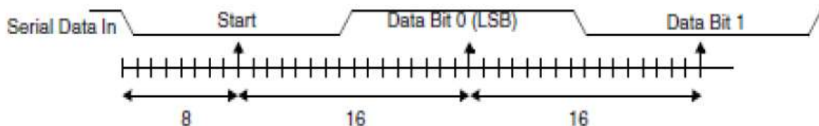
Figure 82. Receiver serial data sampling points
