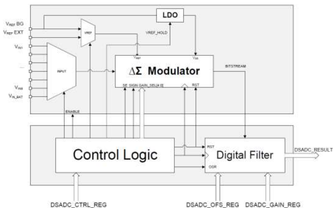
Figure 62. Block diagram of the \Sigma\Delta ADC
