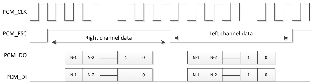
Figure 65. I2S mode
