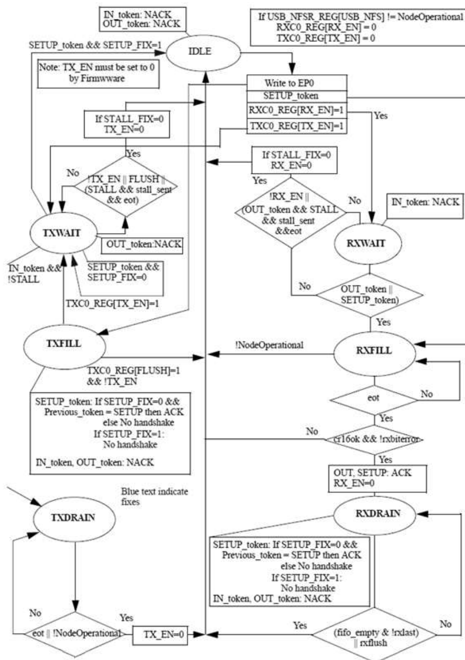
Figure 99. Endpoint 0 operation
