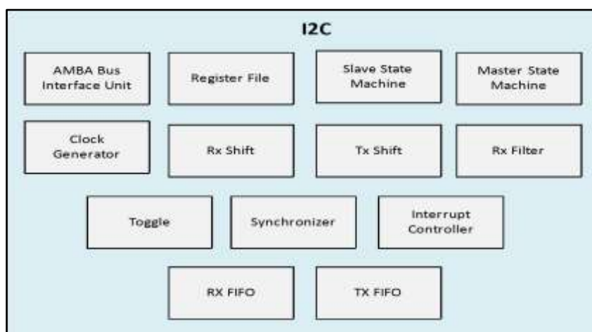
Figure 70. I2C Controller block diagram
