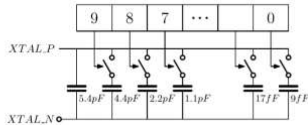
Figure 38. XTAL32MHz oscillator frequency trimming
