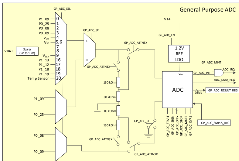
Figure 60: General-purpose ADC block diagram
