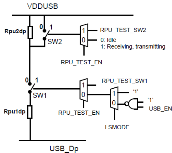
Figure 103. USB_Dp resistor switching
