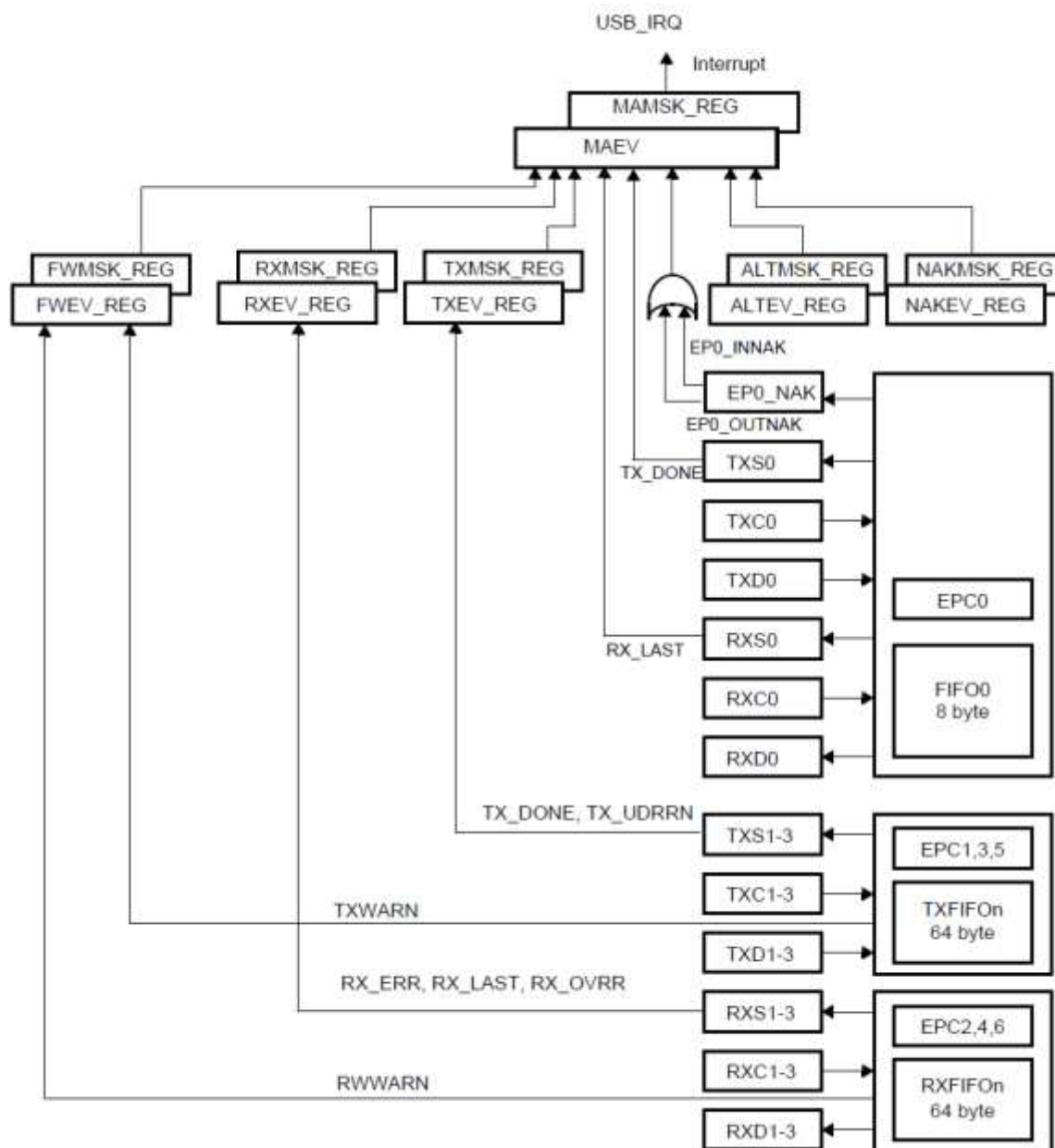
Figure 102. USB Interrupt register hierarchy
