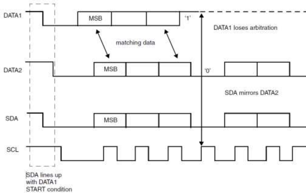
Figure 78. Multiple Master arbitration
