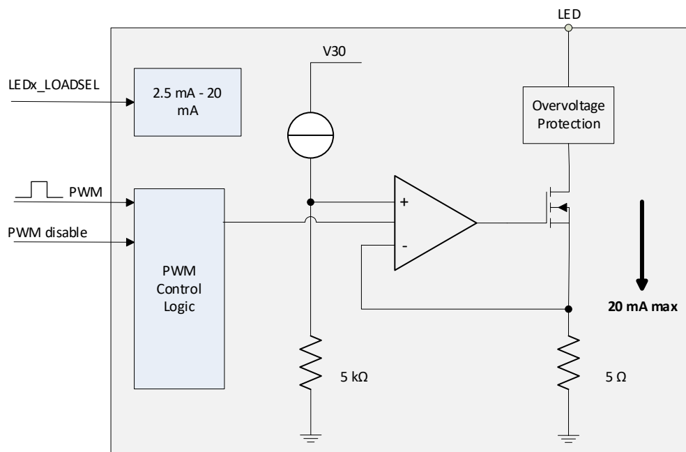
Figure 107. LED Driver block diagram
