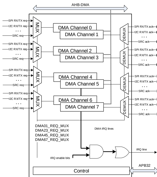
Figure 55. DMA controller block diagram
