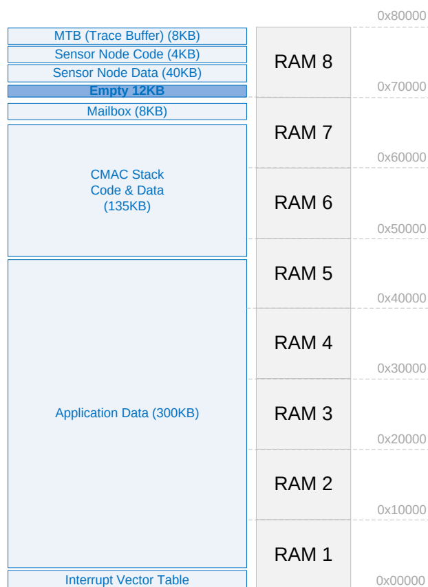
Figure 35. Example of memory segments mapping
