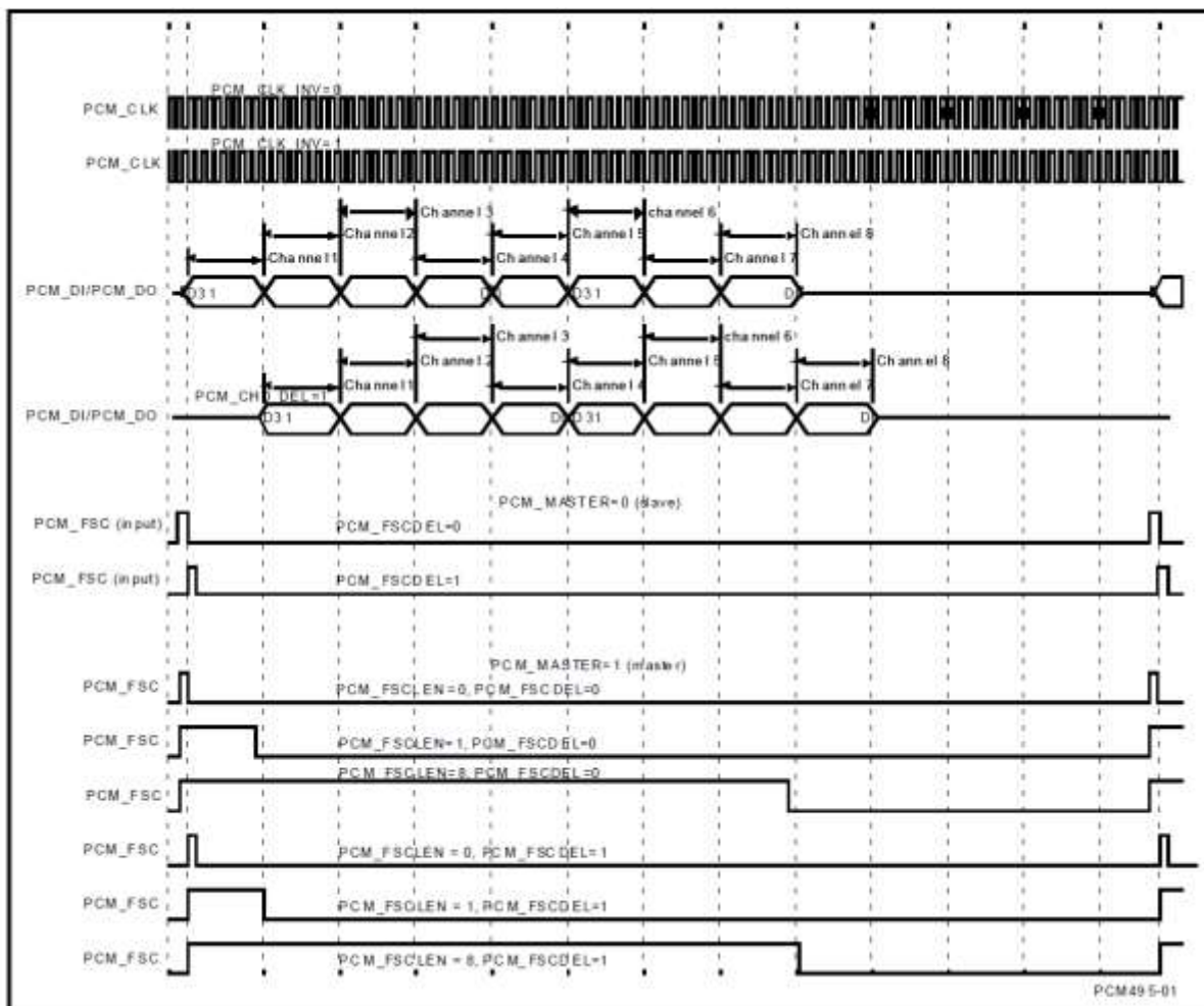
Figure 64. PCM interface formats
