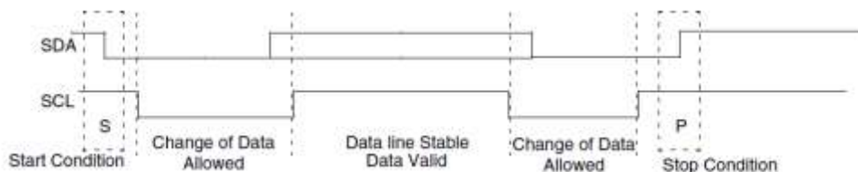
Figure 72. START and STOP conditions
