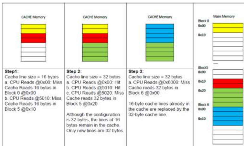
Figure 29. Cache line size reconfiguration example
