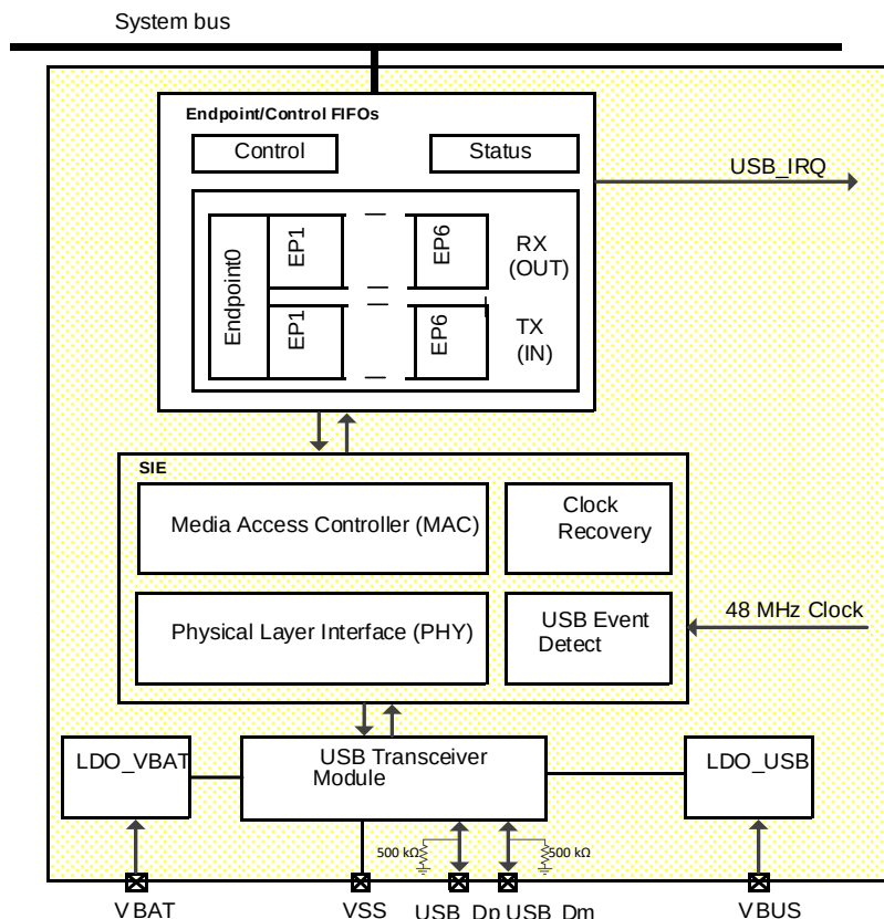
Figure 95. USB Node block diagram
