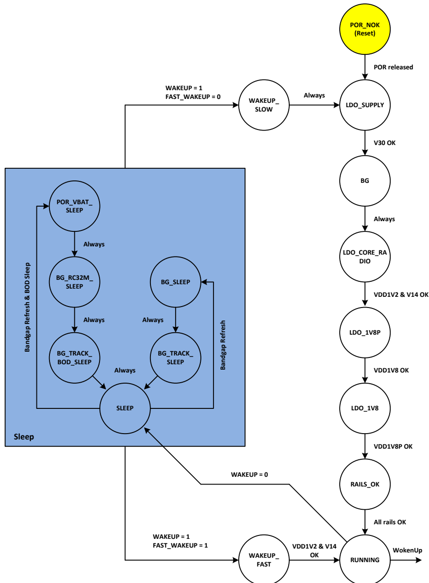
Figure 8. POWERUP, WAKEUP, GOTO Sleep hardware FSM
