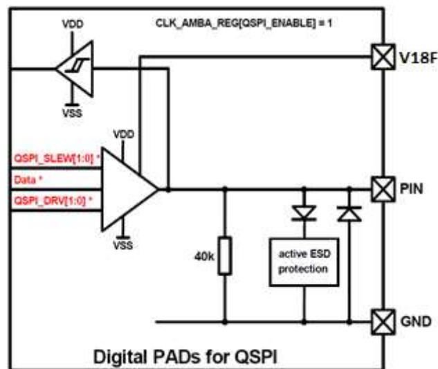
Figure 110. Latching of QSPI pad signals
