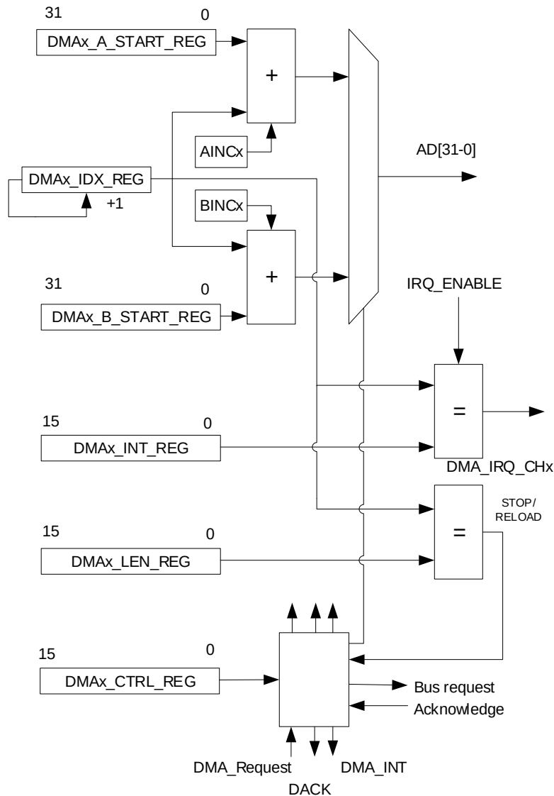
Figure 56. DMA channel diagram
