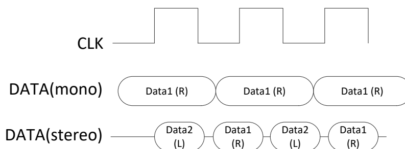
Figure 68. PDM Mono/Stereo formats
