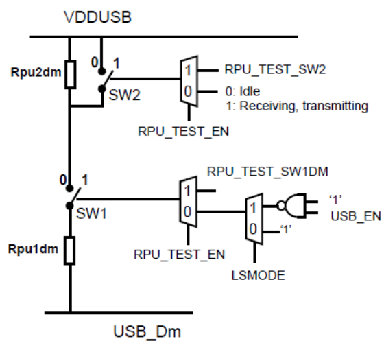
Figure 104. USB_Dm resistor switching
