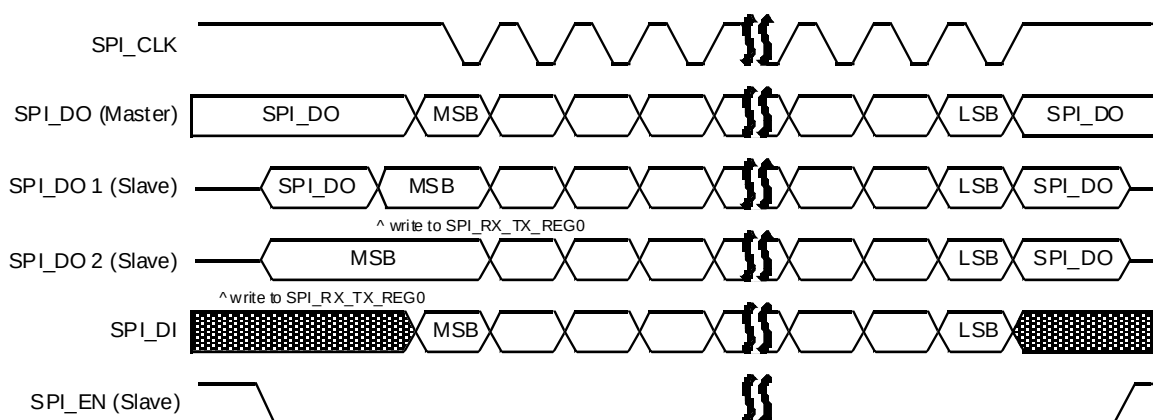
Figure 89. SPI Master/Slave mode 2: SPI_POL=1 and SPI_PHA=0
