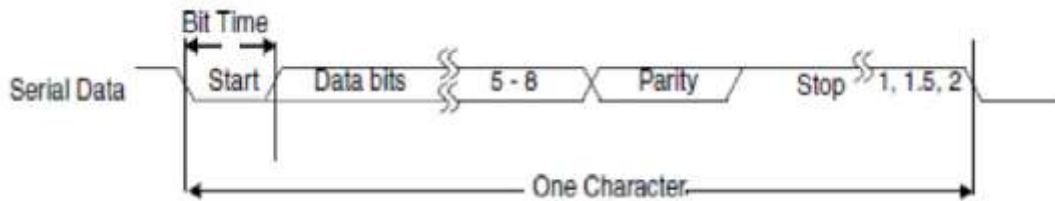
Figure 81. Serial data format
