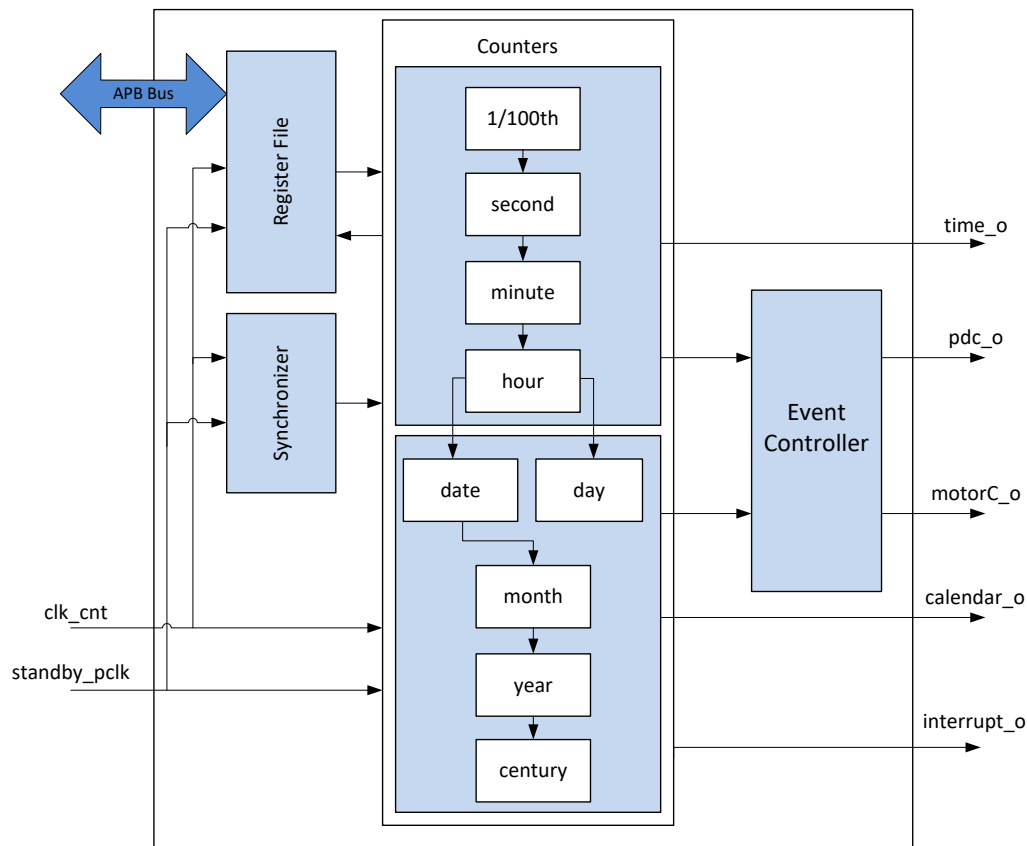
Figure 92. Real Time Clock block diagram
