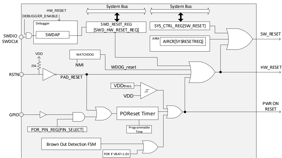
Figure 26. Reset block diagram
