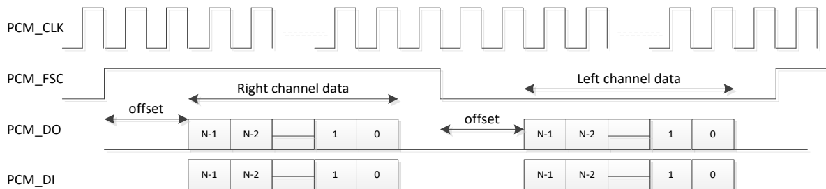
Figure 66. TDM mode (left justified mode)
