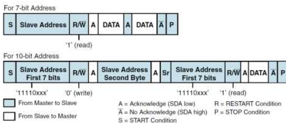
Figure 76. Master-Receiver protocol
