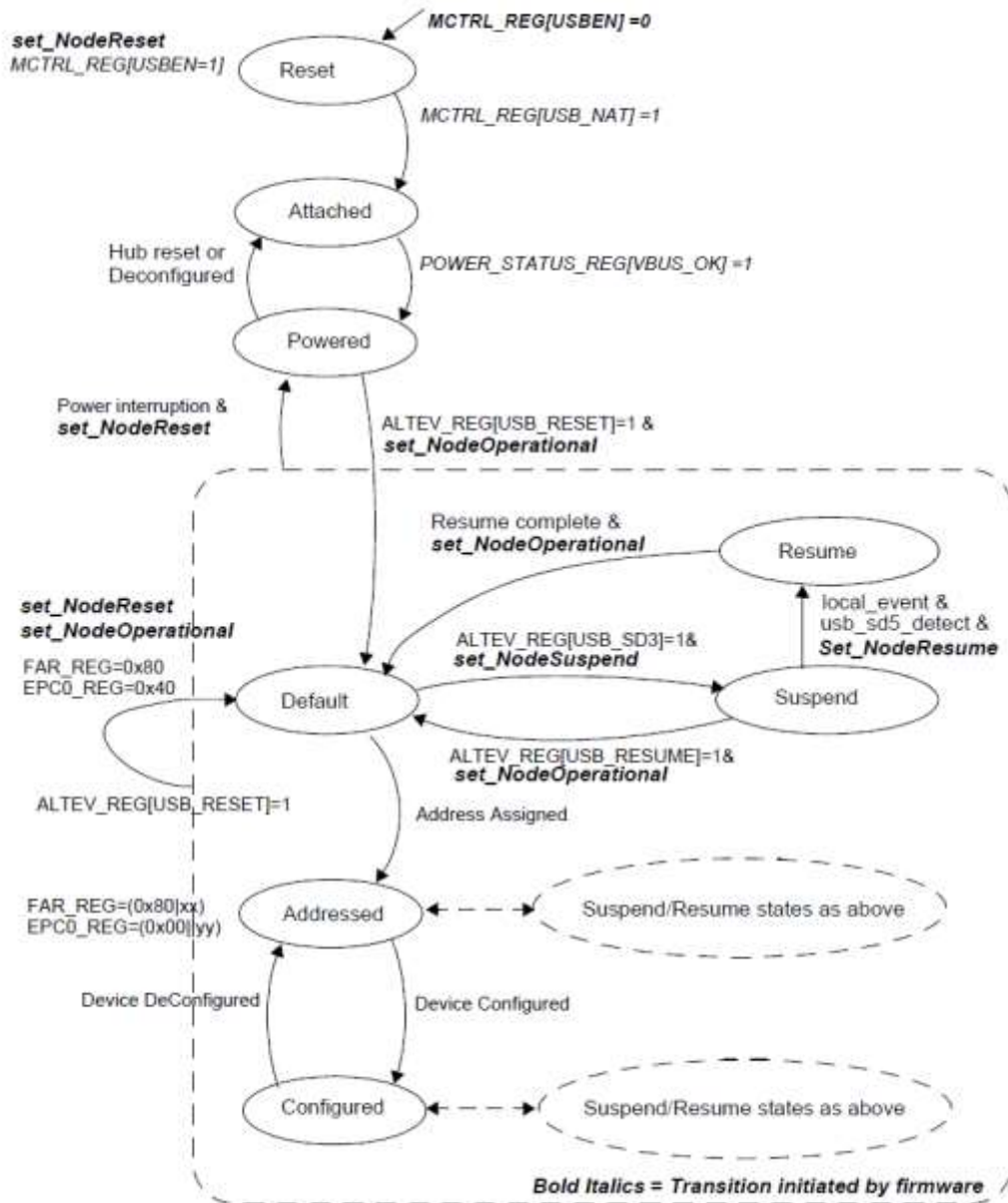
Figure 97. Node Functional State Diagram
