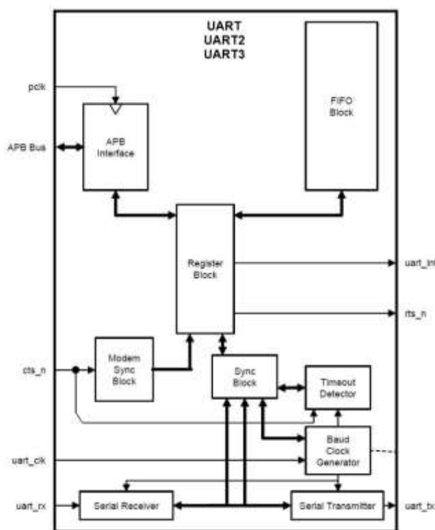
Figure 80. UART block diagram
