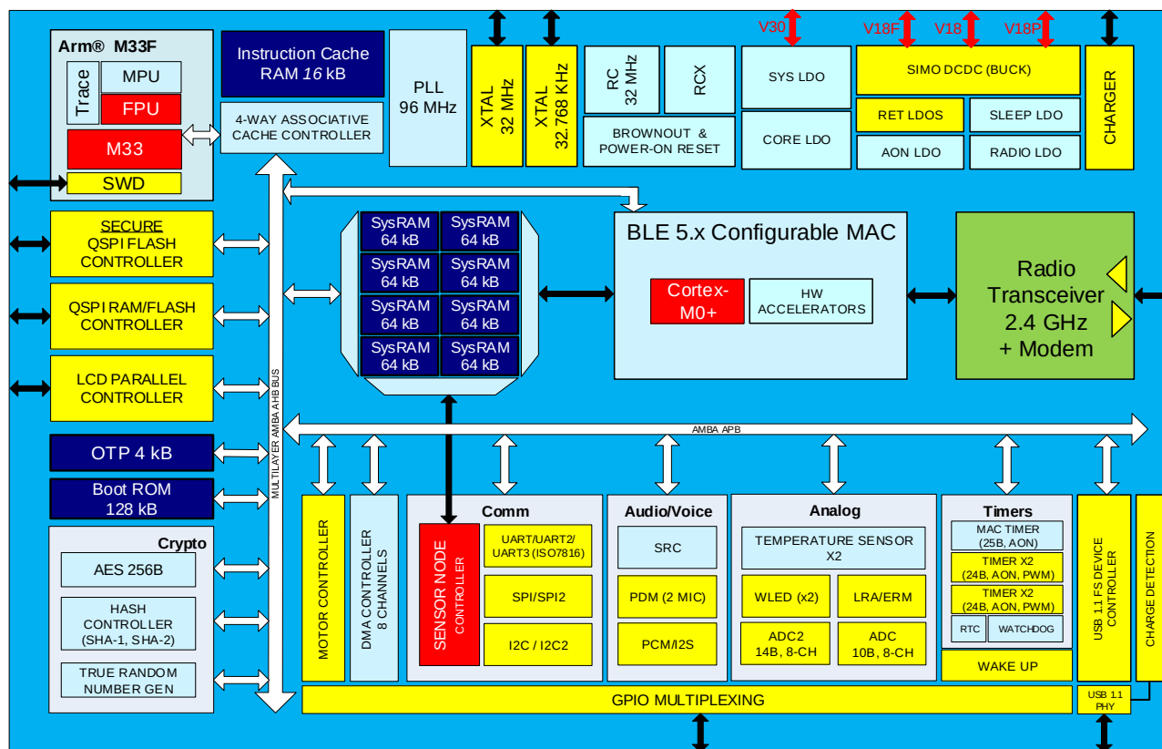
Figure 1. DA1469x block diagram
