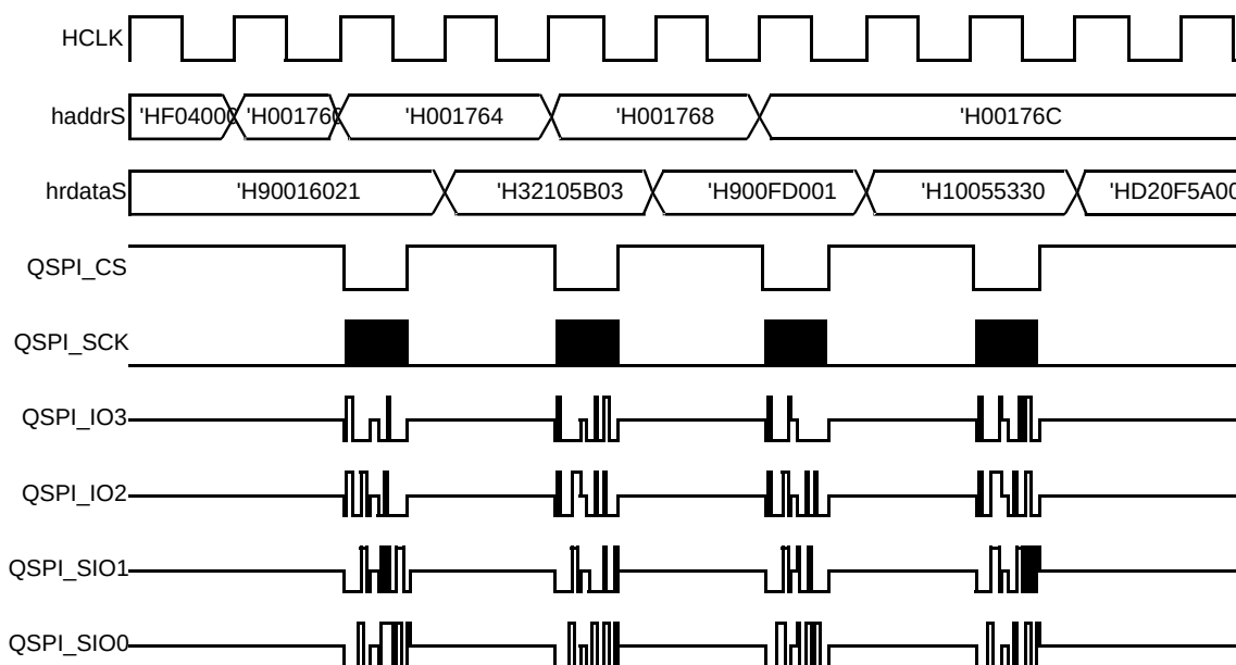
Figure 46. QSPI Split burst timing for low power (QSPI_FORENSEQ_EN=1)
