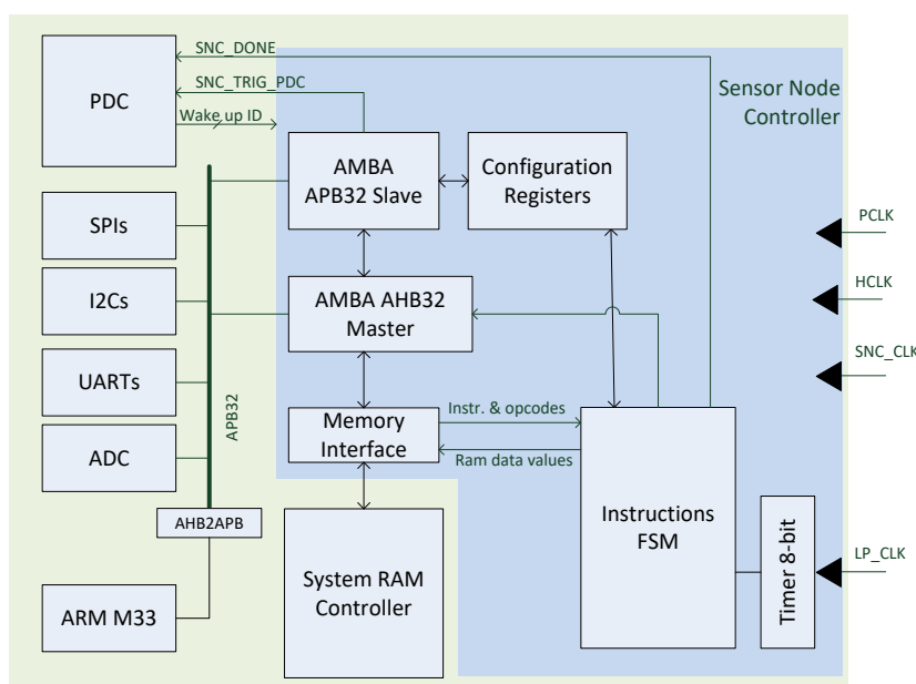
Figure 33. Sensor node controller block diagram
