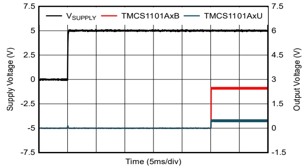
Figure 6-26. Startup Transient Response
