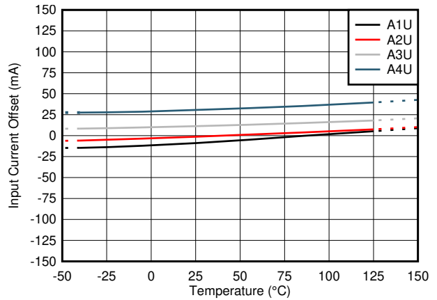
Figure 8-3. Offset Error Drift Across Temperature (U Variants)
