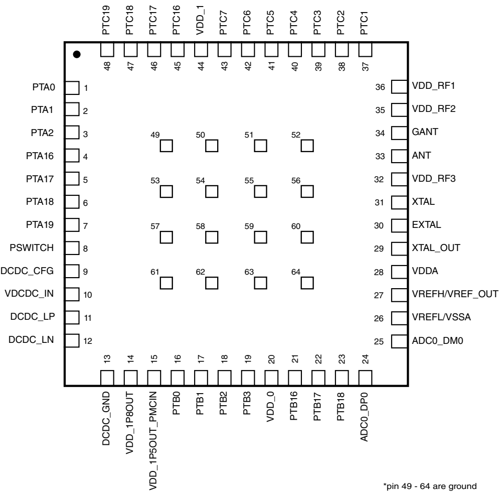
Figure 21. 48-pin LQFN pinout diagram
