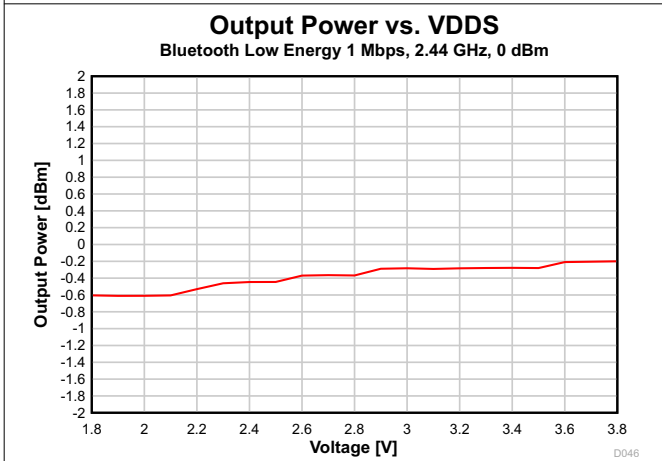
Figure 7-25. Output Power vs. Supply Voltage (VDD5) (Bluetooth Low Energy 1 Mbps, 2.44 GHz)
