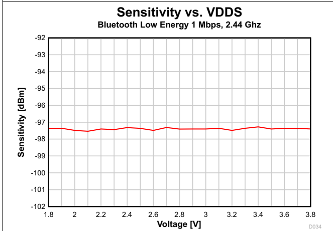
Figure 7-18. Sensitivity vs. Supply Voltage (VDD5) (Bluetooth Low Energy 1 Mbps, 2.44 GHz)
