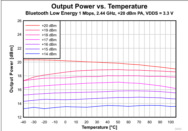
Figure 7-23. Output Power vs. Temperature (Bluetooth Low Energy 1 Mbps, 2.44 GHz, +20 dBm PA)
