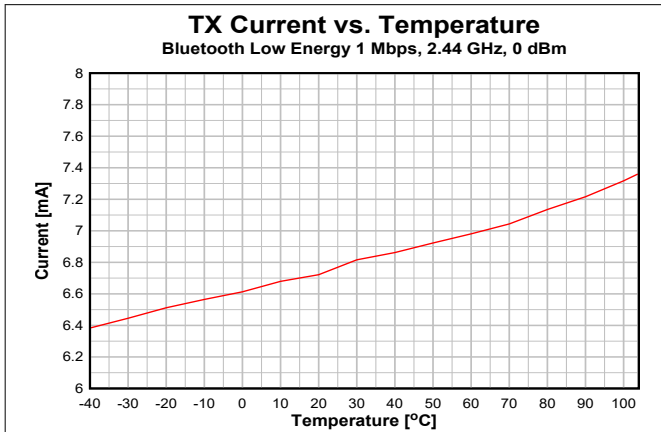
Figure 7-8. TX Current vs. Temperature (Bluetooth Low Energy 1 Mbps, 2.44 GHz)
