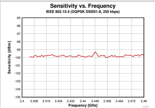
Figure 7-15. Sensitivity vs. Frequency (250 kbps, 2.44 GHz)
