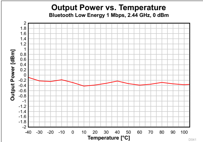
Figure 7-21. Output Power vs. Temperature (Bluetooth Low Energy 1 Mbps, 2.44 GHz)
