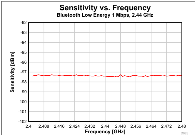
Figure 7-14. Sensitivity vs. Frequency (Bluetooth Low Energy 1 Mbps, 2.44 GHz)
