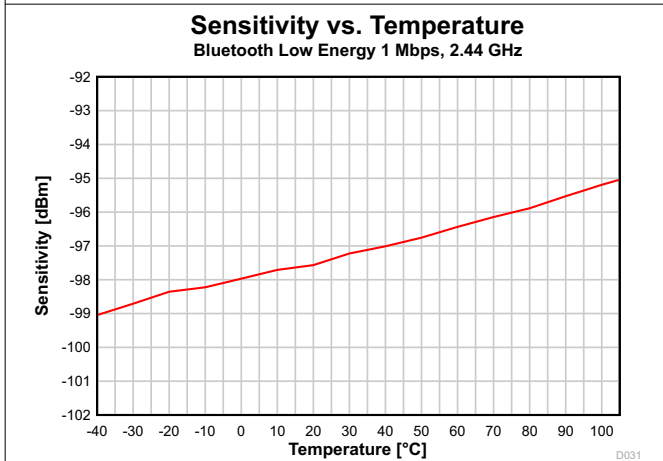
Figure 7-16. Sensitivity vs. Temperature (Bluetooth Low Energy 1 Mbps, 2.44 GHz)
