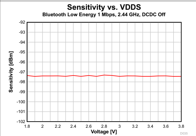
Figure 7-19. Sensitivity vs. Supply Voltage (VDD5) (Bluetooth Low Energy 1 Mbps, 2.44 GHz, DCDC Off)
