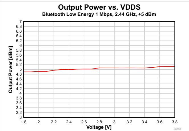
Figure 7-26. Output Power vs. Supply Voltage (VDD5) (Bluetooth Low Energy 1 Mbps, 2.44 GHz, +5 dBm)
