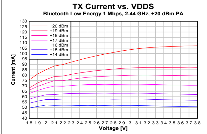
Figure 7-12. TX Current vs. Supply Voltage (VDD5) (Bluetooth Low Energy 1 Mbps, 2.44 GHz, +20 dBm PA)
