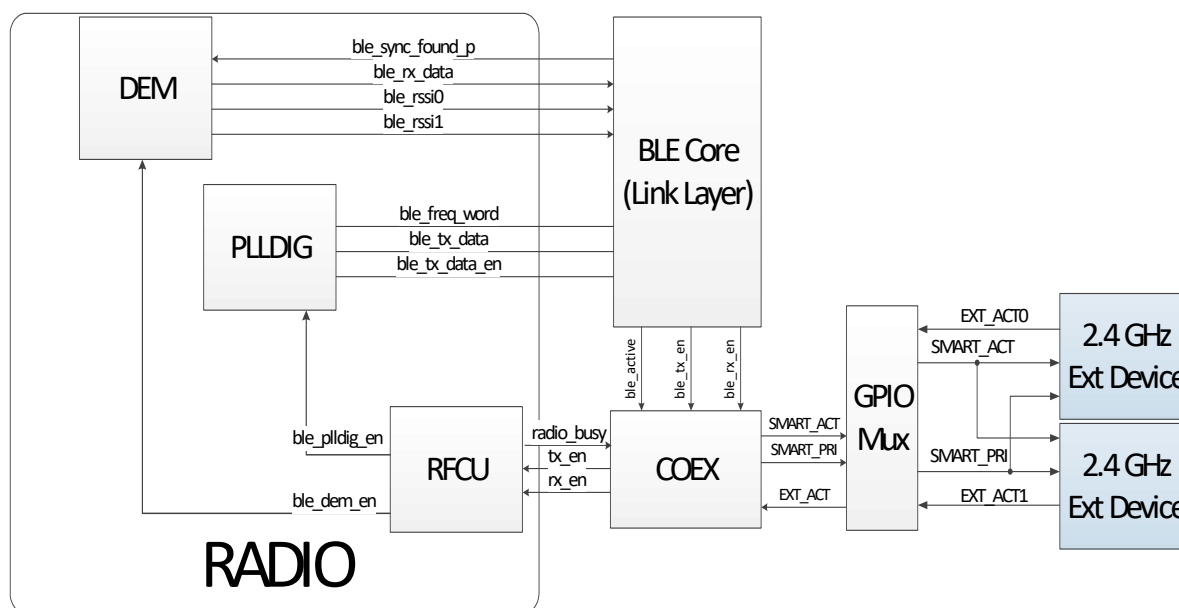
Figure 130: Coexistence interface
