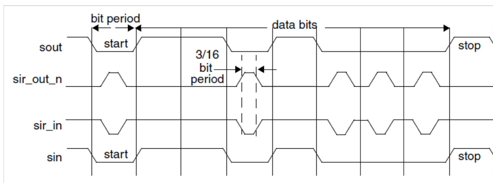
Figure 76: IrDA SIR Data Format
