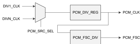
Figure 67: PCM clock generation
