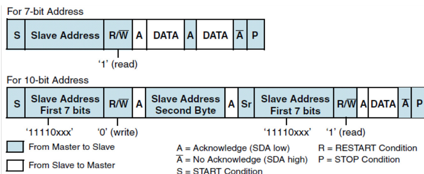
Figure 92: Master-Receiver Protocol
