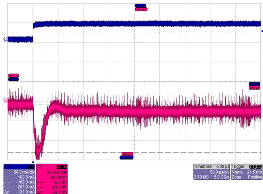
Figure 19: LDO_RADIO loadstep 0 to 35mA (Cload=4.7uF, Vout=1.45V)
