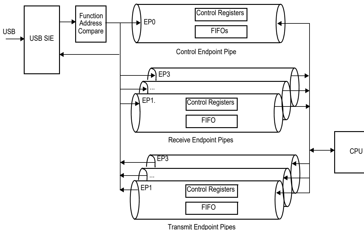
Figure 111: Endpoint Operation
