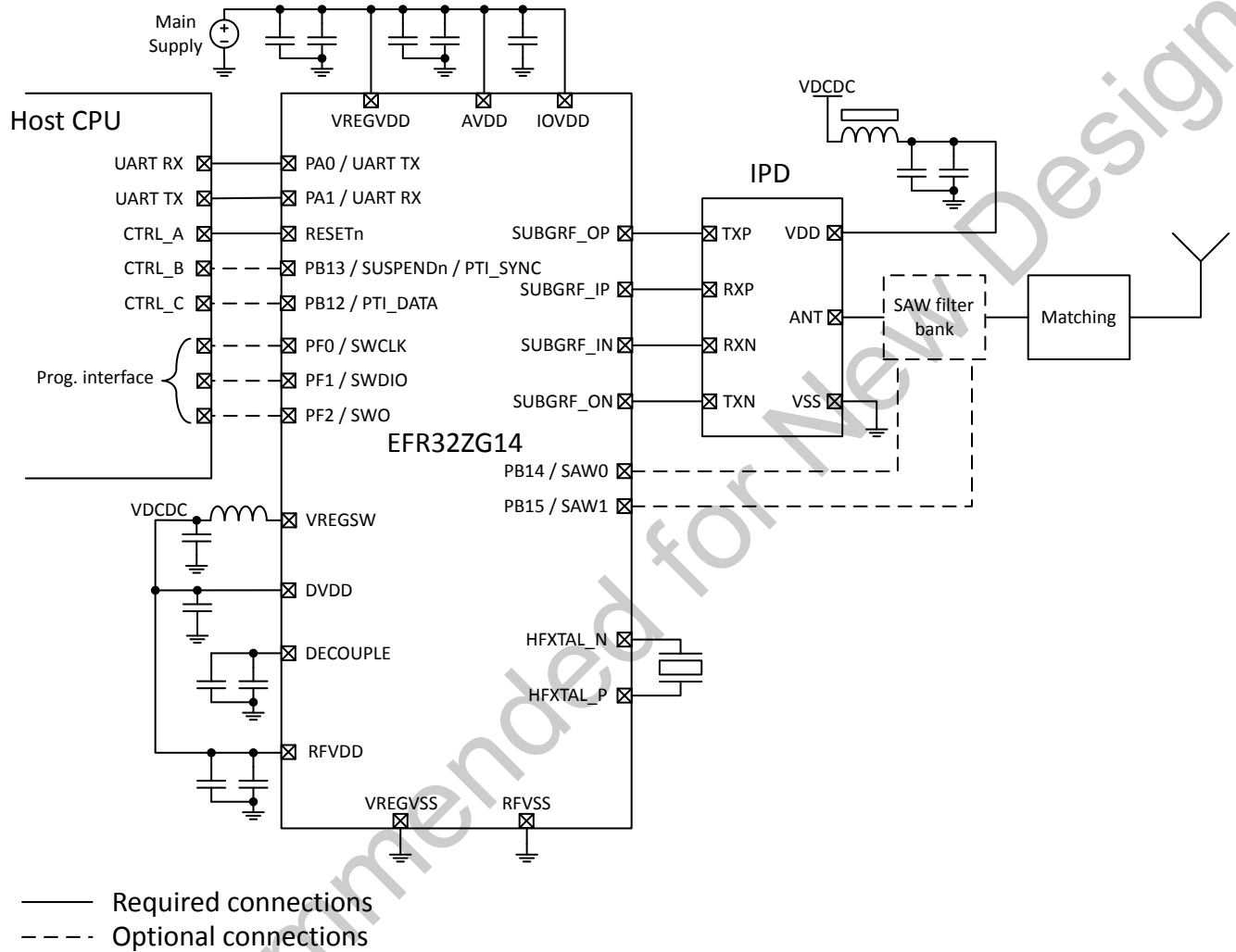
Figure 5.1. Typical System Connections for Z-Wave with IPD
