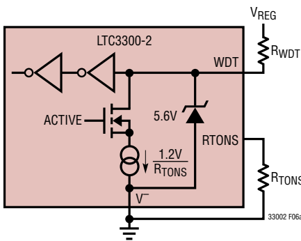
(6a) Watchdog Timer Only (WDT = V^- to Defeat)
