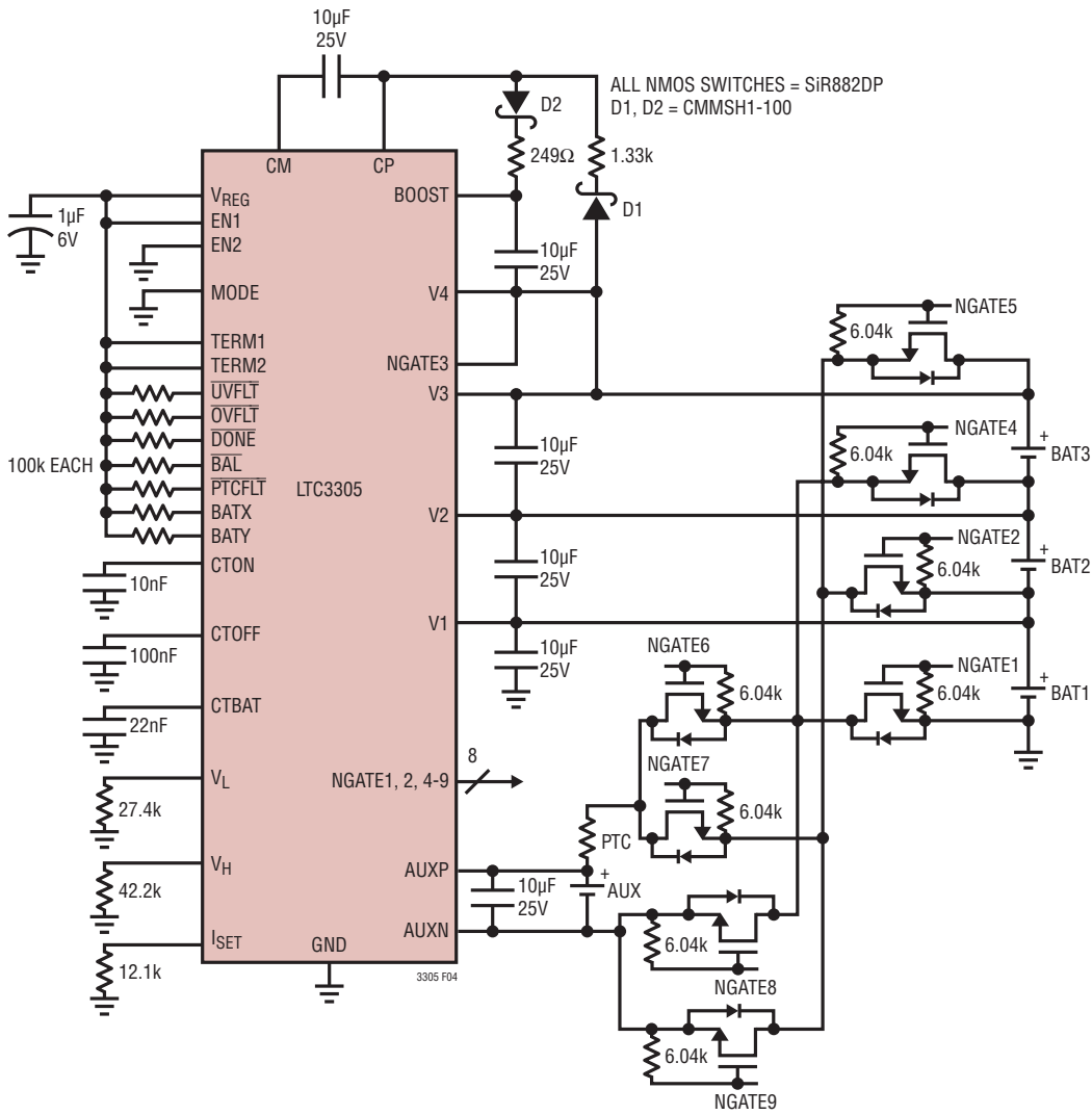
Figure 4. Three-Battery Application Showing External Switch Arrangement
